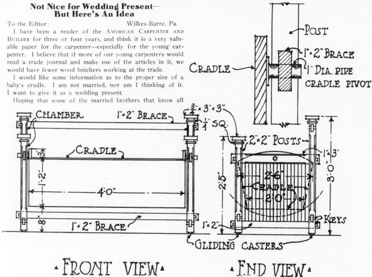
Working Drawings of Craftsman Crib or Baby's Cradle.
