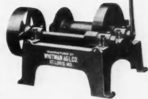
SULTAN BELT-DRIVEN HOIST WITHOUT ENGINE
