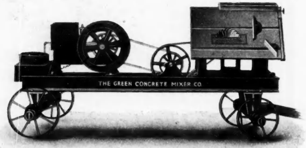
The Green Steel Truck with Saw Table.
