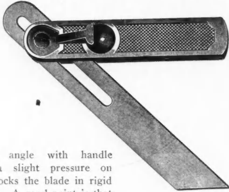
The Blade Locks in Any Position.
