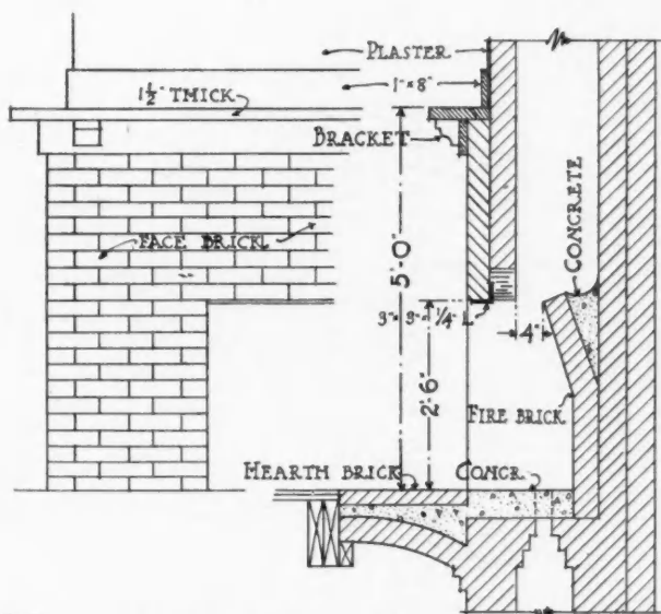
HALF ELEVATION & SECTION OF FIRE PLACE
