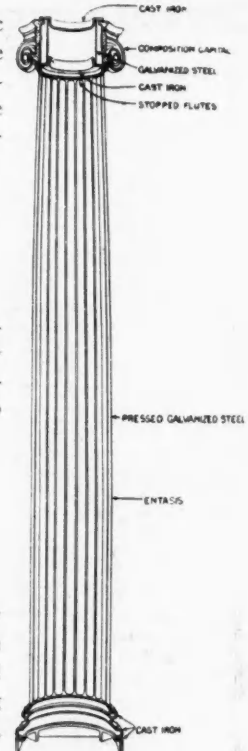
Construction of Union Metal Column.
