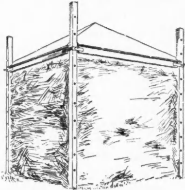
An Adjustable Roughage Stack Cover—Roughage, stacked in the hog lot where it can be easily thrown down for feeding sows in winter, should be protected by a cover. A simple roof adjustable on four corner posts is satisfactory.
