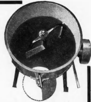
Inside view of drum showing door for unloading
