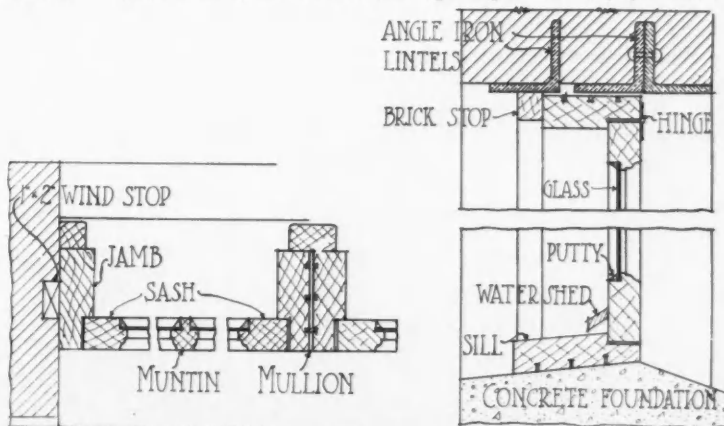
Fig. 2. Details Separated and Labeled for Clearness.
