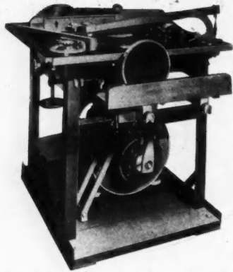
THE SULTAN COMPLETE PORTABLE SAW RIG For all around efficiency this machine is unsurpassed. Is equipped with five H. P. Sultan Sawing Engine. The Saw has gravity blower to take saw-dust or shavings away from engine at all times.
