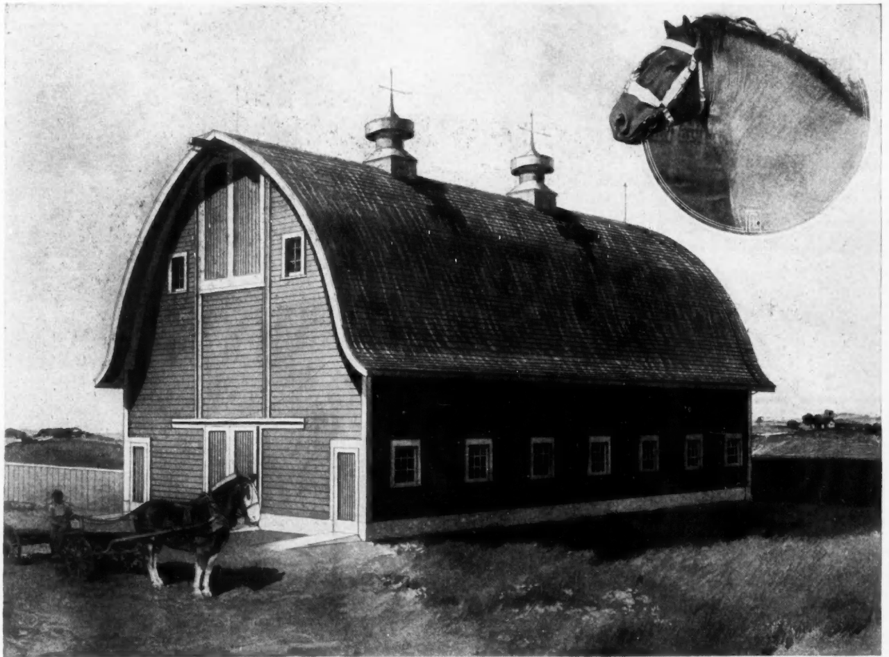
A businesslike Gothic-roof design to stable 16 cows and 14 horses. Overhead litter carrier runs through both stables. Size on ground, 70 by 36 feet. We can furnish complete set of blue-printed working plans and typewritten specifications for only $10.00 per set. When ordering, ask for Design A282.
