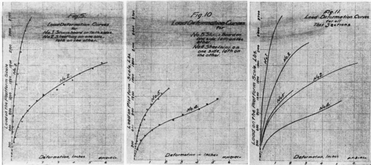
Graphic Records of Tests Showing Superior Strength of Stucco Board to Resist Wind Pressure Strains when Used in Place of 3/8-Inch Sheathing.
