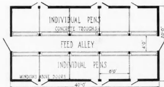
Floor Plan of Hog House Built by Harold Dunnett.
