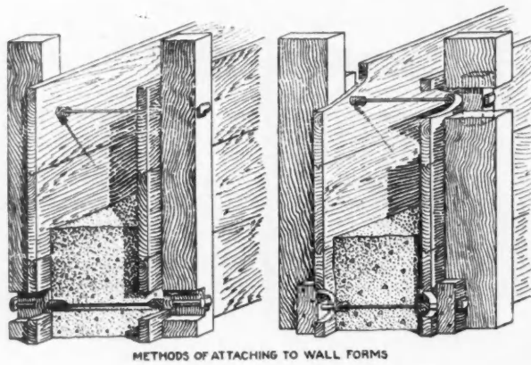
Various Applications of "Tyscru" as Form Tiers, Anchorage, and Reinforcement.
