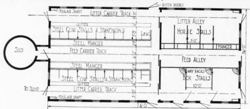
Floor Plan of Gambrel Roof Barn. Design No. A284.
