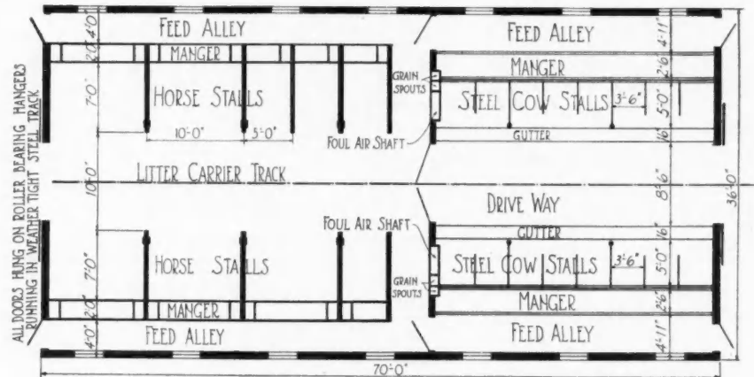
Floor Plan of Gothic Roof Barn. Design A282.
