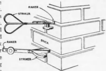
Showing Method of Using Combination Raker and Striker.
