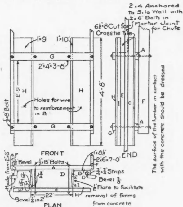
FRONT AND END ELEVATIONS AND PLAN VIEW OF WOOD FORMS FOR CONTINUOUS CONCRETE DOOR FRAME
