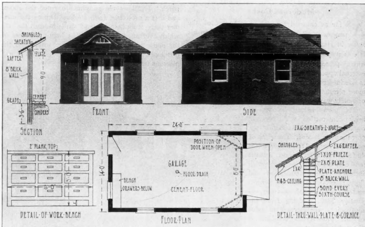
Trim Little Garage Giving Plenty of Space for One Large Car. Walls Are Built of Face Brick Backed with Common Brick. Notice Detail of Handy Bench with Drawers Below. Hip Roof with Exposed Rafters Is Artistic Feature. The Doors Are of the Type to Slide Inside Around the Corner.
