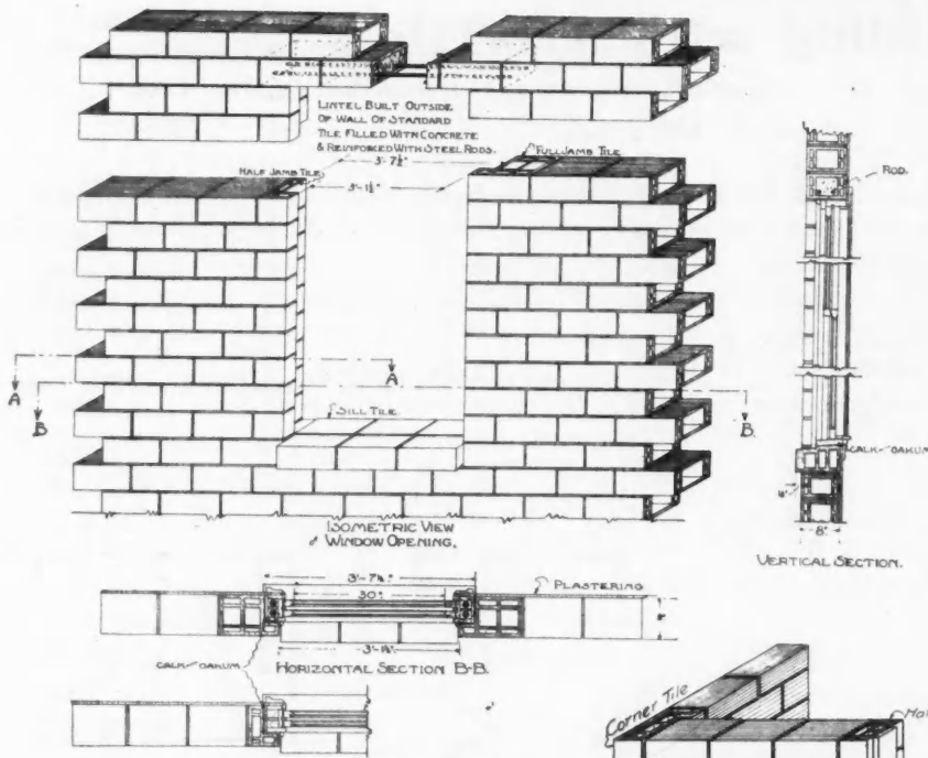
Details of Window Openings in Sinclair House.
