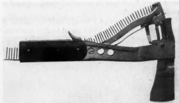
An Automatic Lathers' Hammer, Showing How Nails Are Fed.
