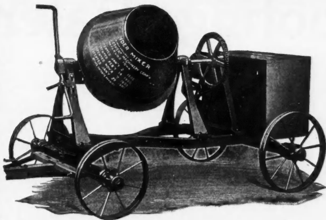
MODEL 15 —The mixer for light work—capacity 5 to 6 cubic feet per batch. Can be equipped with auxiliary hoist. Mixes mortar as well as concrete. 3 H. P. Wonder Gas Engine requires least attention of any ever designed for mixer service. Equipped with Gear Tilt if desired.
