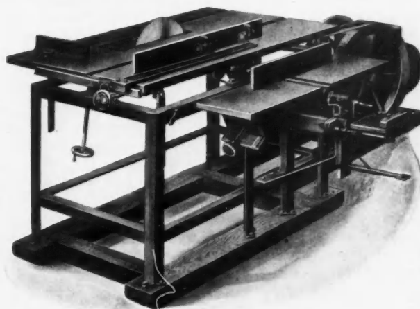
Light But Strong Portable Power Woodworker.
