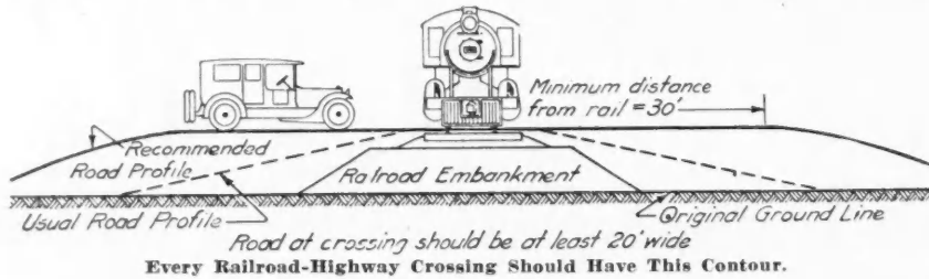
Every Railroad-Highway Crossing Should Have This Contour.
