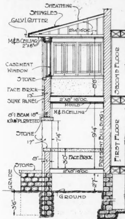
PORCH SECTION A A
