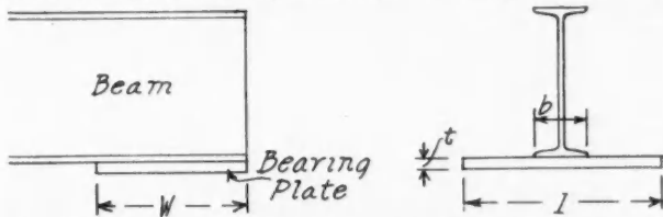
Dimensions of Beam Flange and Bearing Plate Referring to Following Formulae for Plate Thickness.
