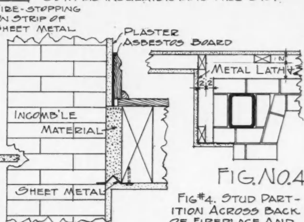
FIG. NO. 3 FIG. #3. SHOWING SUPPORT OR FIRE-STOPPING AROUND CHIMNEY AND PROTECTING WOODWORK. FIG. NO. 4 FIG. #4. STUD PARTITION ACROSS BACK OF FIREPLACE AND AROUND THE ENDS OF CHIMNEY BREAST, SHOWING PROPER METHOD OF ARRANGING STUDS.
