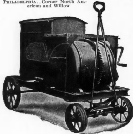
Lansing No. 5 "half-sack" batch mixer.
