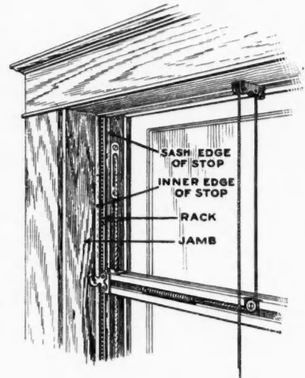
Details of New Shade Adjuster.
