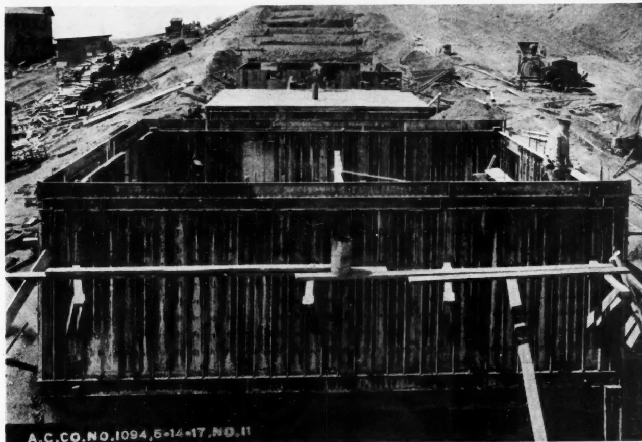
Progress Photo Taken Seven Days After View at Top of Opposite Page.
