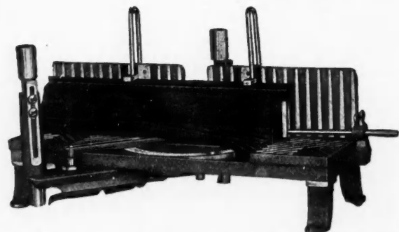
Improved Miter Box, Showing Crown Moulding Held in Place by Stock Gauges and One Length Gauge in Position.
