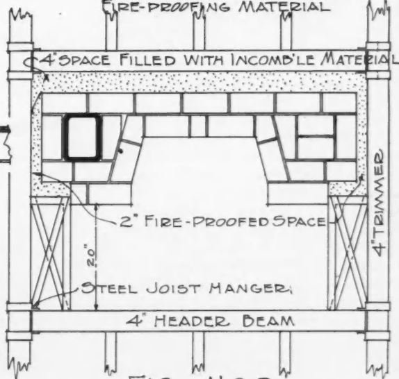
FIG. NO. 2 FLOOR FRAMING AROUND A SINGLE FIREPLACE. NOTE FILLING BETWEEN FRAMING AND BRICKWORK, WHICH SERVES BOTH AS INSULATOR AND FIRE-STOP.
