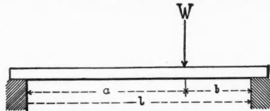
Simple Beam with Concentrated Load at Any Point.
