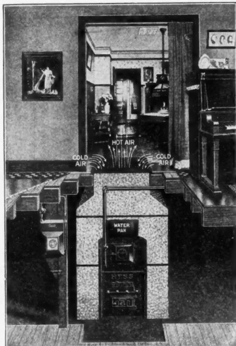
The Hess Welded Steel Pipeless Furnace One large register delivers heat and draws cold air from the floor back to the furnace
