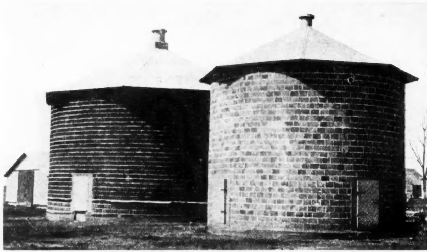
Ten Thousand-Bushel Round Corn Crib and 8,000-bushel grain tank, both of hollow clay tile on the farm of R. C. Head, near Jefferson, Iowa.
