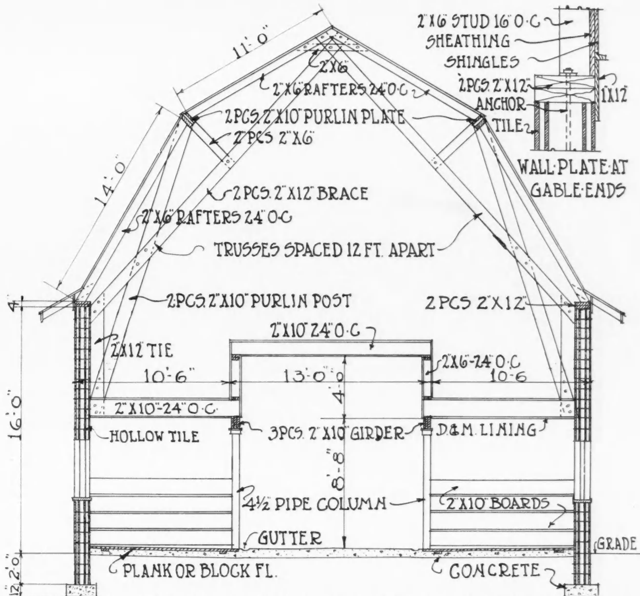
Section Thru Hollow Tile Horse and Cow Barn, Showing Framing for Self-Supporting Roof. The tile walls extend clear up to the eaves. The purlin braces come down to the floor joists and are tied to the ends of the truss chord above at the plate line by means of two pieces of 2 by 12 for each truss. This takes the outward thrust away from the top of the tile wall.
