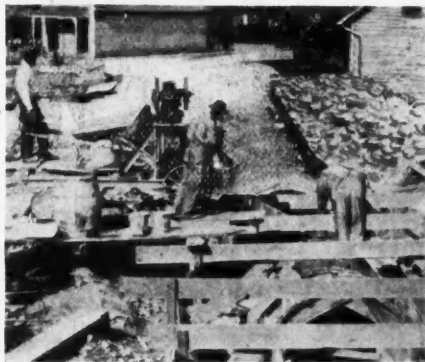
Half Bag Archer Mixer Delivering Direct Into Forms on Sewer Conduit Work
