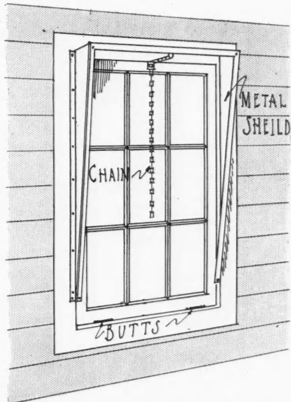
A Ventilating Stable Window, hinged at the bottom to swing in. The metal shields at each side throw all the draft up when window is opened, protecting animals from direct draft.
