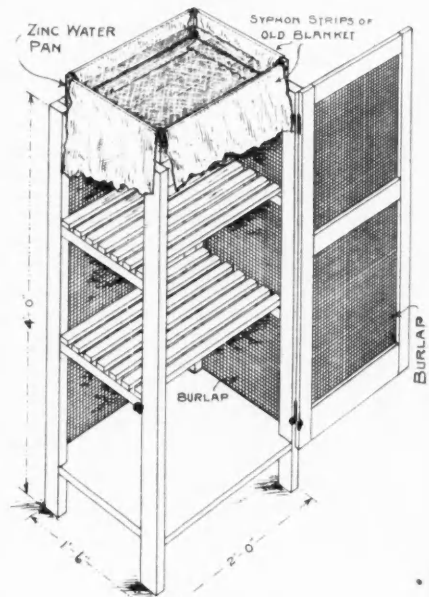
Iceless Cupboard.
