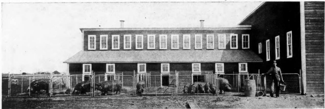
Example of Steel Gate Panels for Pig Yards on the Weiland Farm, Near Canistota, S. Dak. These 7 pens each measure 7 by 21 feet. All panels are mounted on removable posts for cleaning or changing the sizes of these hog runs. Each pen has its own gate.
