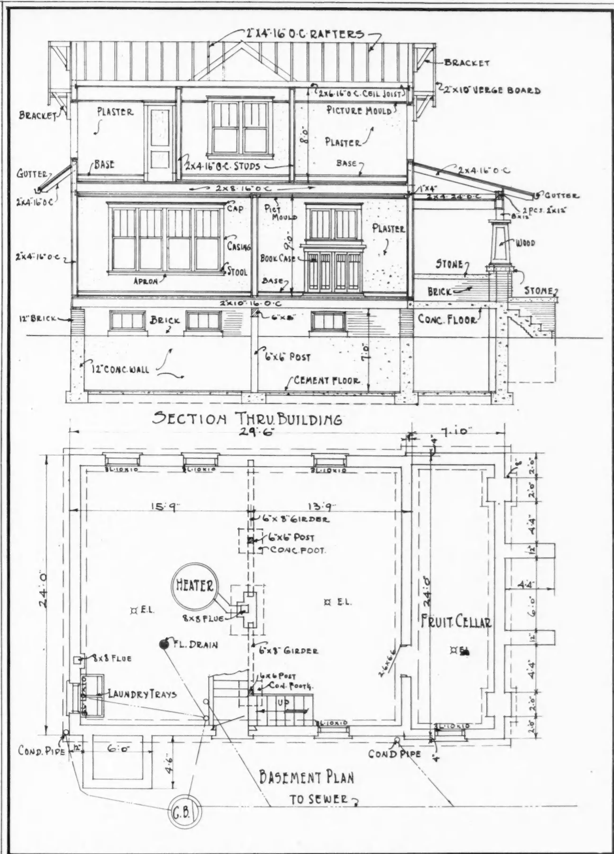
PLANS OF SIX ROOM ONE AND ONE HALF STORY RESIDENCE SCALE 1/8" = ONE FOOT SHEET NO 3
