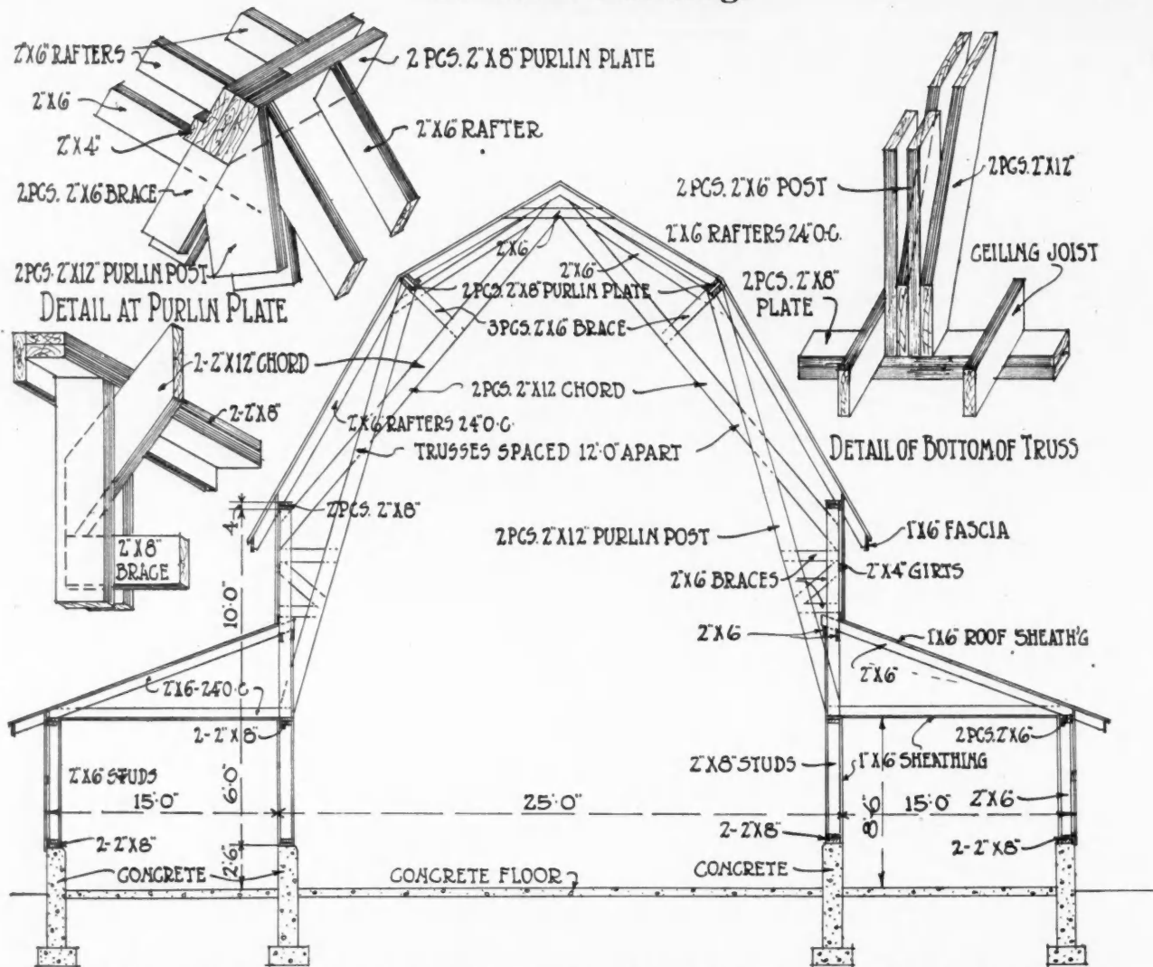
Details of Hay Storage and Horse Barn, Illustrated in Farmstead Group, Plate 8. The high center part is the hay mow and will hold an immense quantity of packed down hay. The horses are stabled in the shed wings along each side. Standard plank frame construction is used for supporting the high roof, trusses being spaced 12 feet apart. Instead of being tied across the bottom of the structure as usual, the side wings brace these trusses from the outside to prevent the feet of the trusses from spreading.
