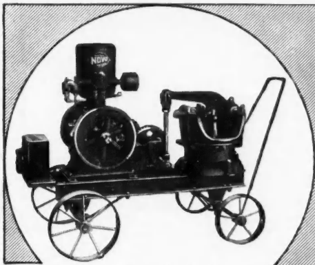
Figure 335—Novo Diaphragm Pumping Outfits, either skid or truck mounted in several sizes, single or double pumps.
