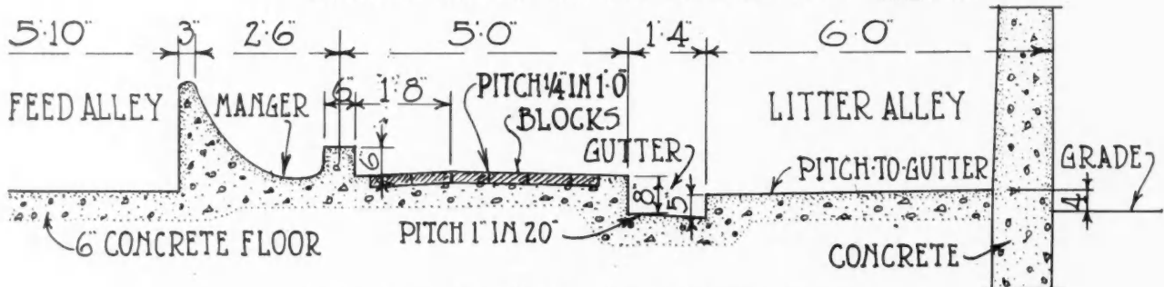
Details of Concrete Stable Floor Arranged for Cows to Face In.
