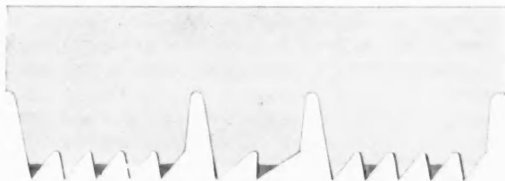
Tooth Detail of New Double Duty Saw.
