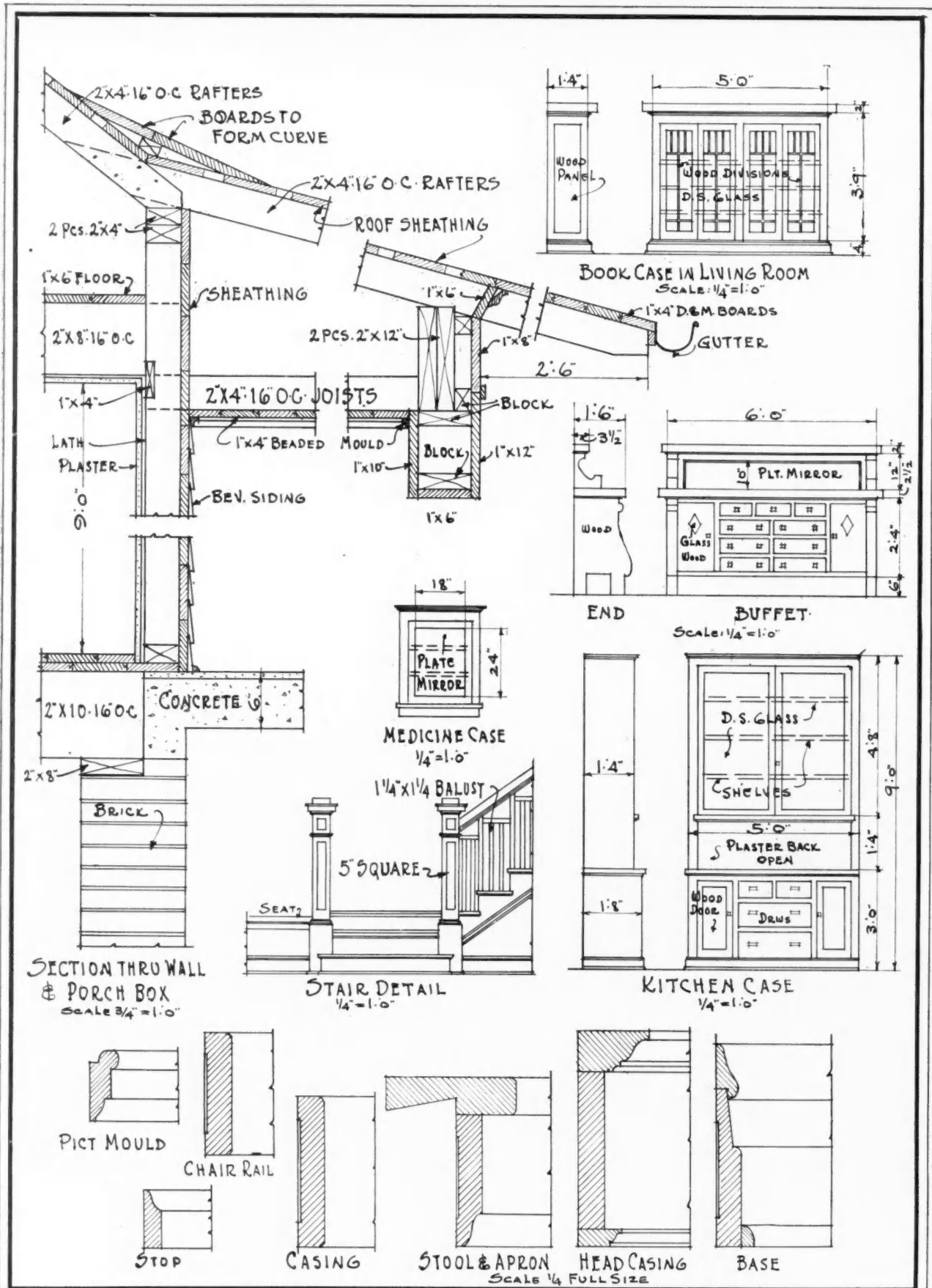
PLANS OF SIX ROOM ONE AND ONE HALF STORY RESIDENCE SCALE AS NOTED ABOVE SHEET NO 4
