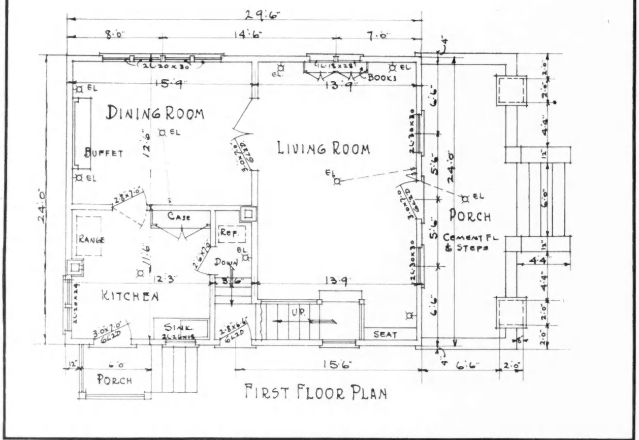
PLANS OF SIX ROOM ONE AND ONE HALF STORY RESIDENCE SCALE 1/8" = ONE FOOT SHEET NO.2
