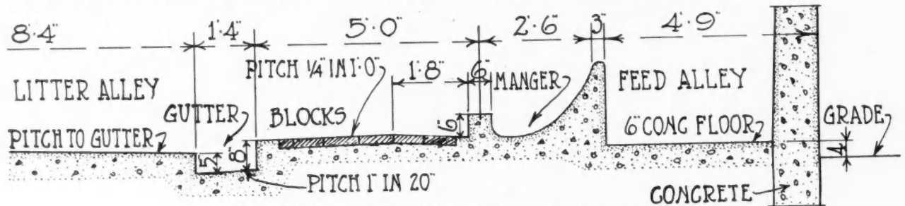
Details of Concrete Stable Floor, Cows Arranged to Face Out.
