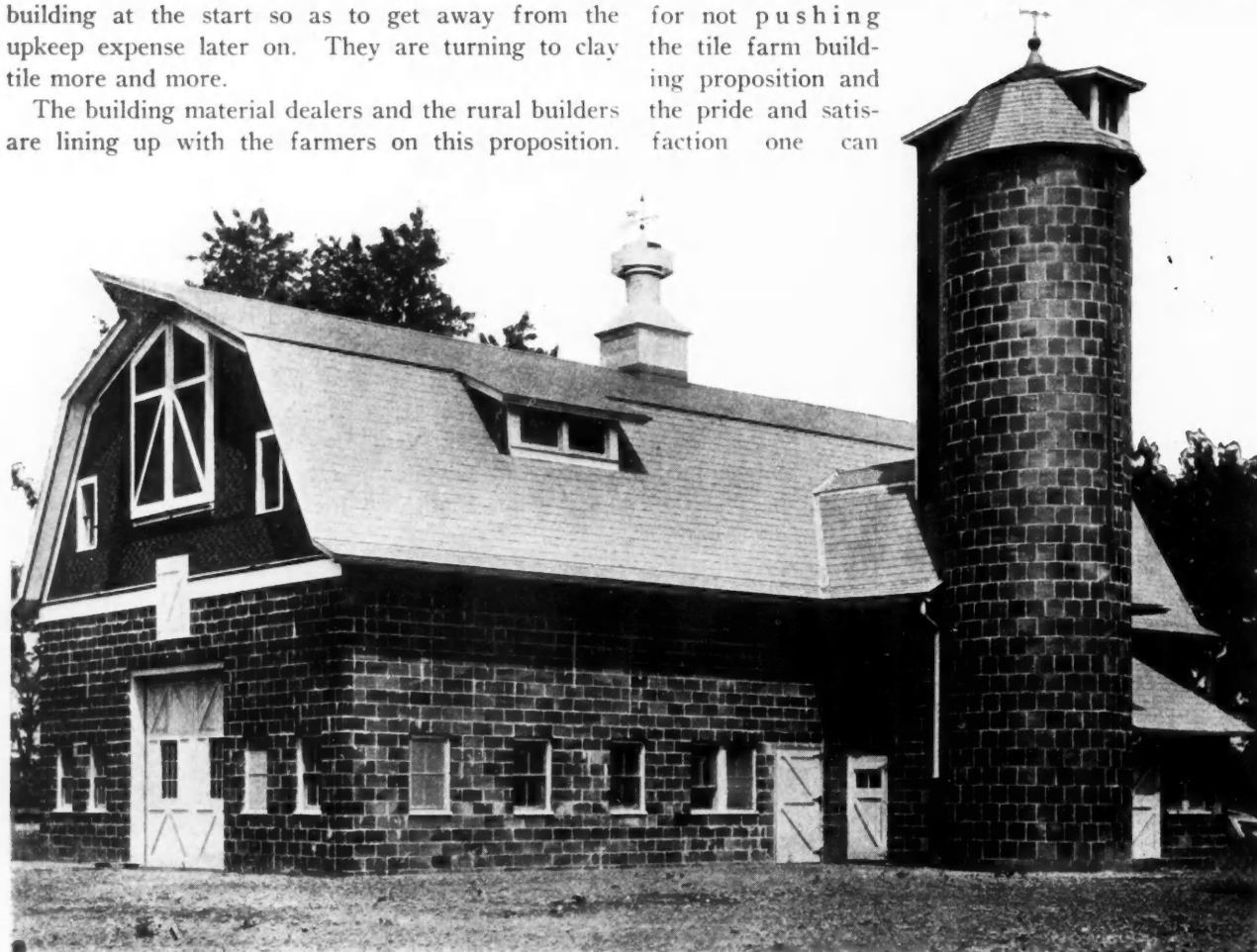
Photograph of Extra Well Designed Tile Horse and Cow Barn, with attached silo and milk house on Phoenix Brothers' Farm, near Bradford, Ill. The tile runs to the eaves and the roof is covered with slate.
