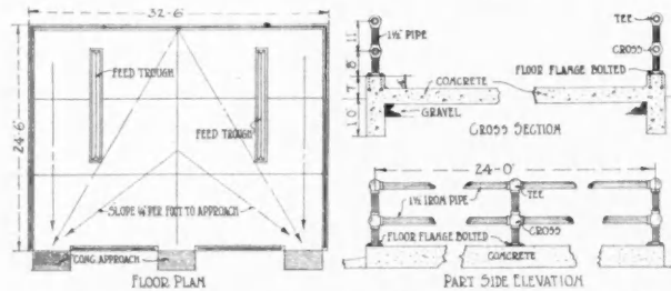
A Show Ring Hog Feeding Floor of Concrete and Iron Pipe.
