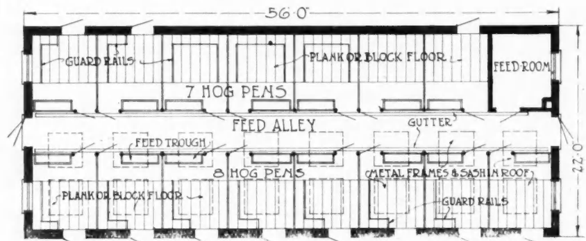
Floor Plan of Community Hog House with tile walls and skylight roof windows, illustrated below.
