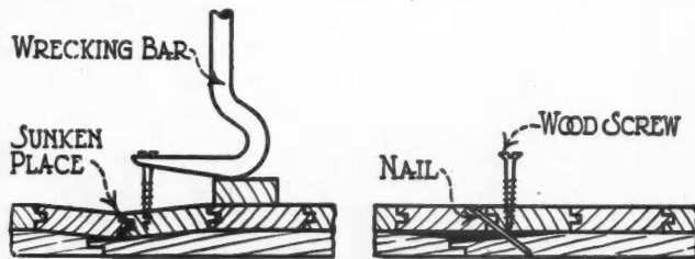
A Sunken Floor Board Can Be Lifted and Secured in Place by This Method Without Making a Big Job of the Repair.
