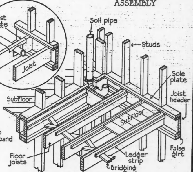
FIG. 23 FRAMING JOIST UNDER BATHROOM
