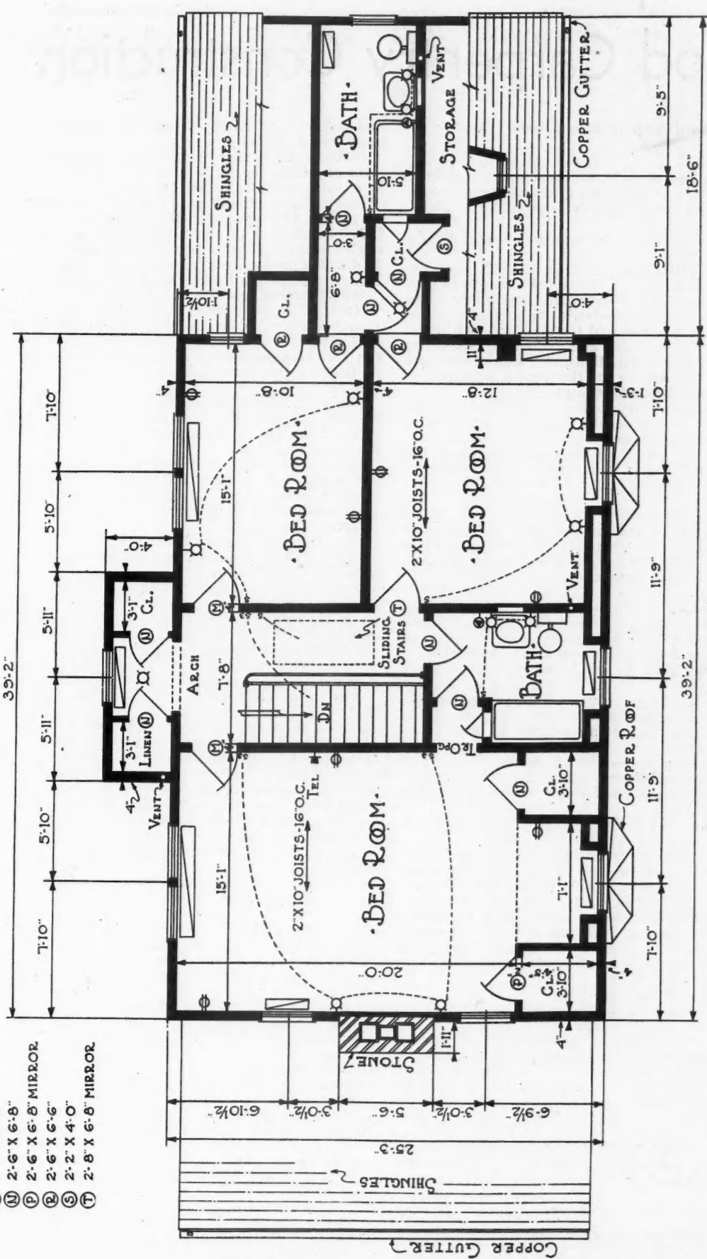
1. SECOND-FLOOR PLAN. SCALE 1/8" = 1'-0"
