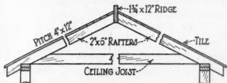
Extra size ridge board supports Spanish tile.
