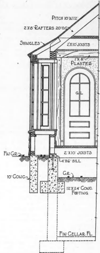
SECTION BB SCALE 1/4"=1'-0"
