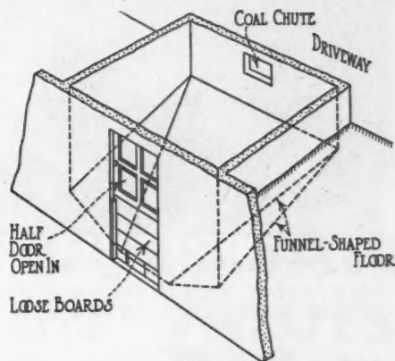
Gravity does the work in this sloping floor coal bin.
