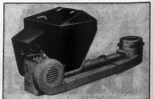
New automatic stoker especially designed for household use.
