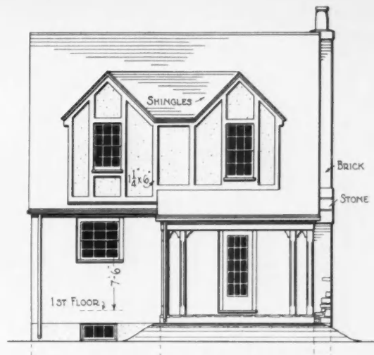
REAR ELEVATION
