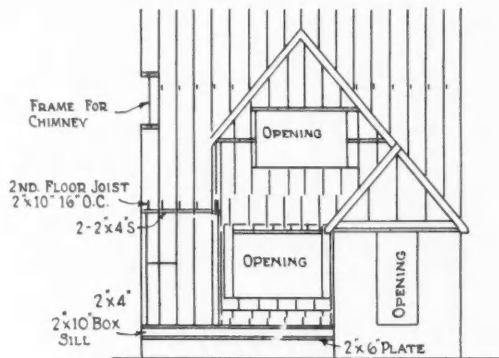
← FRONT WALL FRAMING →
