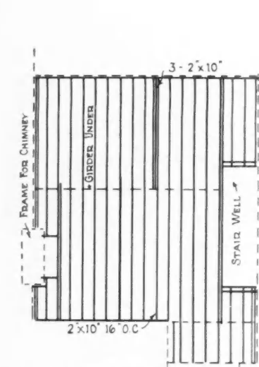
← 1ST. FLOOR JOIST FRAMING →
