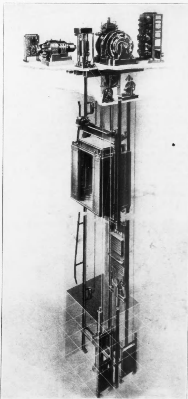
Drawing showing how a typical signal control elevator installation would look if it could be seen without enclosing hatchway walls.
