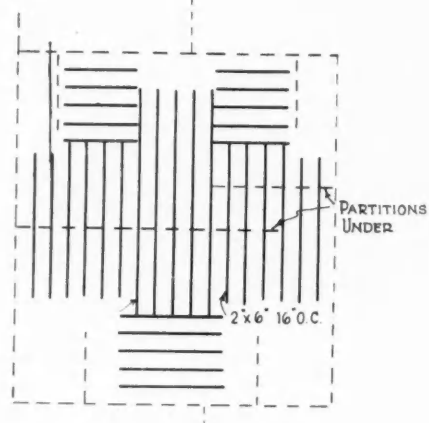
← CEILING JOIST FRAMING →
