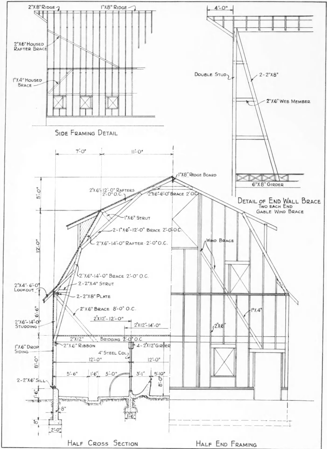
Section through Big Barn showing self-supporting plank-frame roof, also end bracing to resist wind pressure. See two preceding pages for photo and plan.
