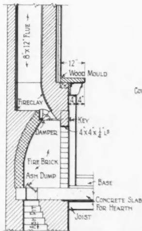
SECTION AT CENTER
