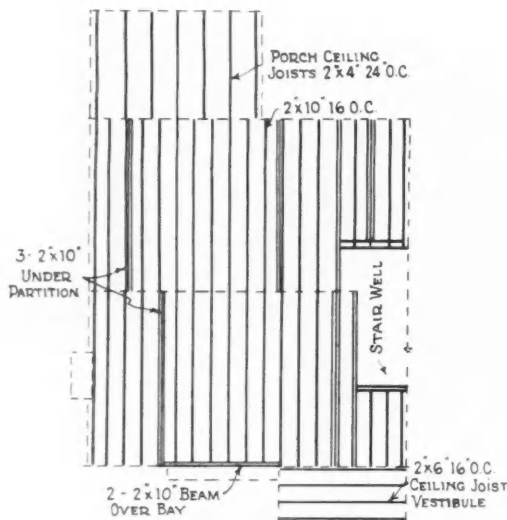
← 2ND. FLOOR JOIST FRAMING →
