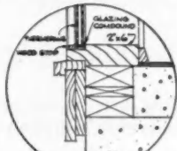
SILL SECTION-B-B
