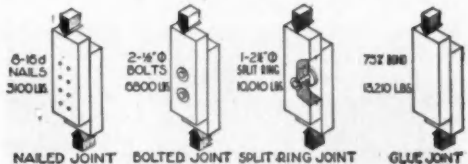
VARIOUS types of joints discussed in text on the previous page. At left are 2x6's fastened with the common nailed joint; next are 2x4's fastened with two 1/2-inch bolts; the third illustrates a timber connected joint with one 2 1/2-inch ring imbedded between two 2x4's. The fourth illustration shows a glued joint with two 2x4's lapped eight inches. This latter joint tested by far the strongest. Drawings on joints and barn roof at left courtesy Weyerhaeuser Sales Co.
