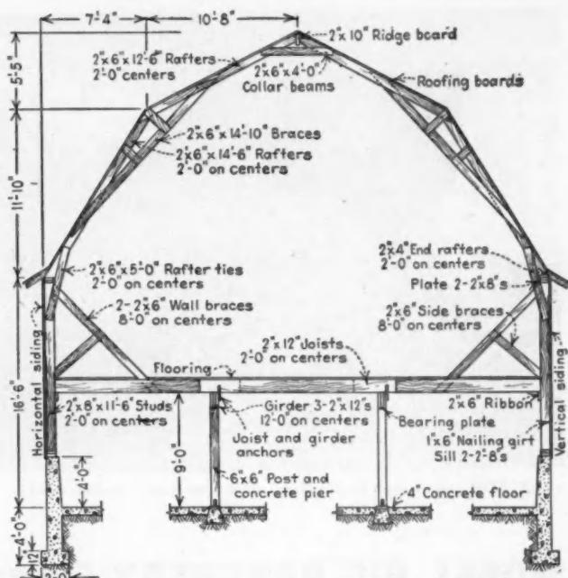
HIGH resistance to wind is the feature of this gambrel roof designed by engineers at Kansas State College. Studs and joists are doubled on 8-foot centers at wall braces
