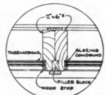
MULLION SECTION-F-F
