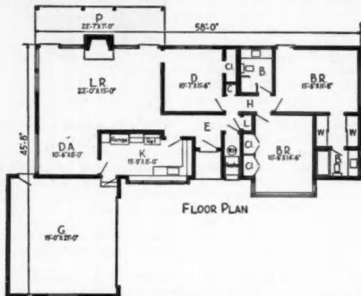
FLOOR PLAN provides a layout of rooms with good circulation to various zones
