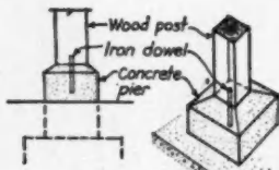
Method of fixing wood post to concrete.
