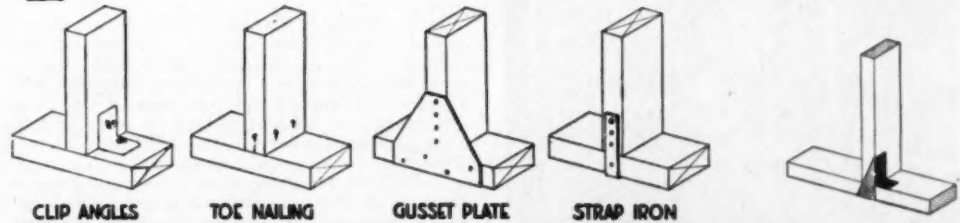
FOUR methods of improving what are commonly toenailed joints. The conventional toenailed joint is shown second from the left. The Timber Engineering Company's newly-developed Trip-L-Grip anchor, made in six different shapes, is at the right
