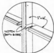
NOTCH JOINT
