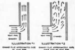
DIAGRAM of effects of oversize chimney
