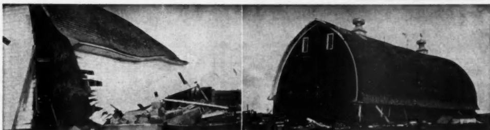
FAILURE of an inadequate masonry block foundation was the main cause of extensive wind damage to this barn. Masonry block walls are only as strong as their weakest mortar joint. There are very few, if any, building codes which would permit unbraced walls of this length, yet there is no hesitancy in building long barns without bracing walls with partitions or buttresses
