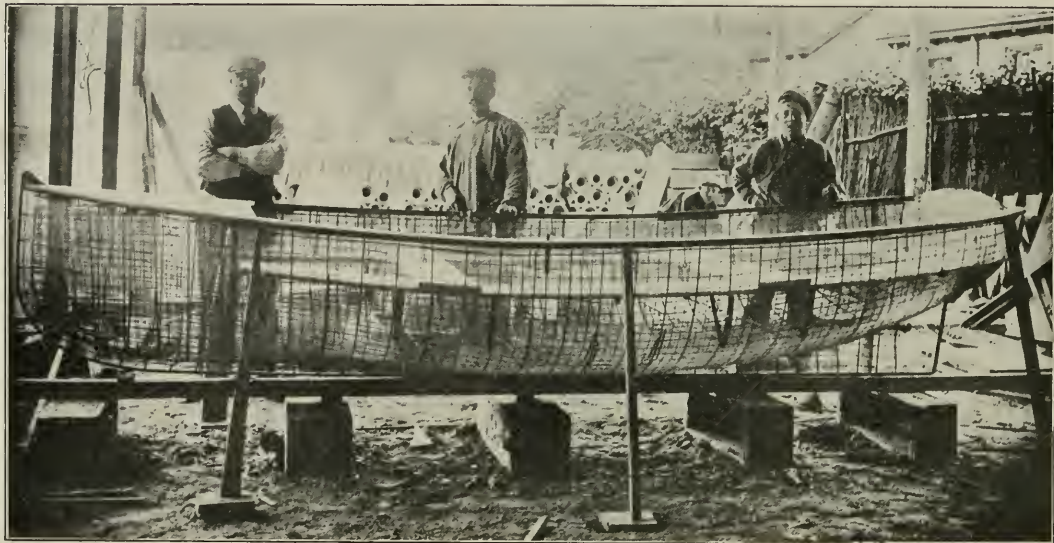
Framework of Motor Boat Ready for the Concrete
