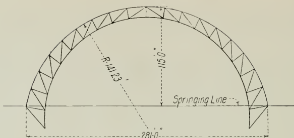
Fig. 2—Sketch of Original Timber Arch Center
