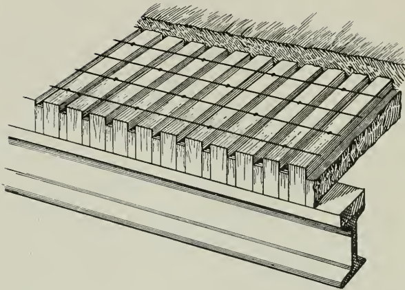
Fig. 1, Showing Method of Laying Floor
