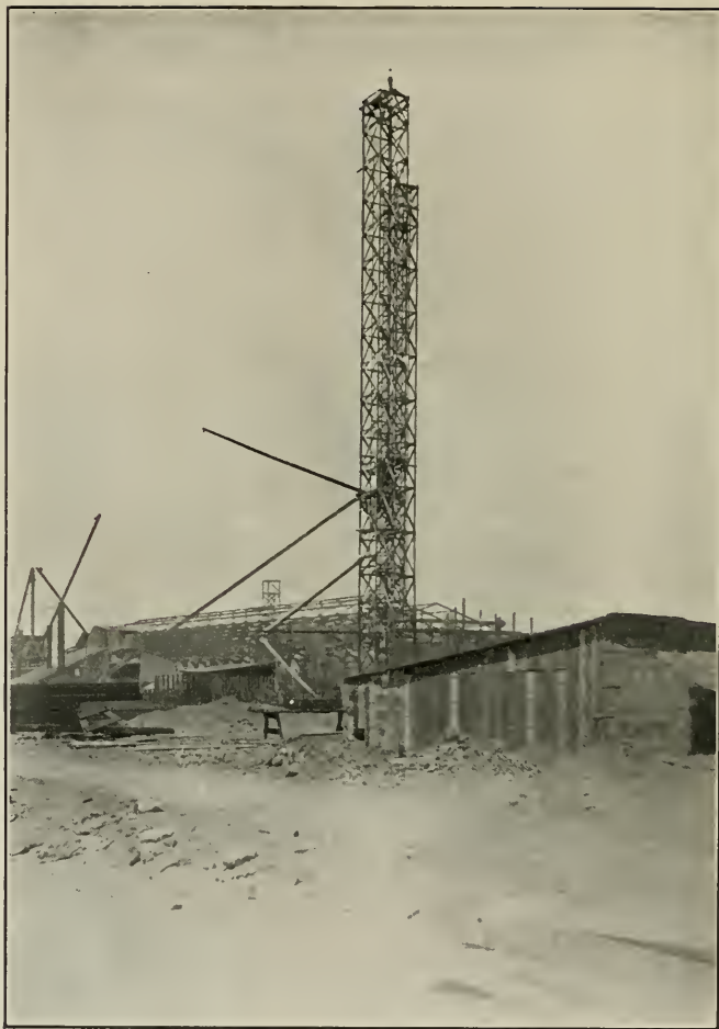
Government Warehouse under construction at Fort Mason, Cal. Ferrolite Company, Contractors.
