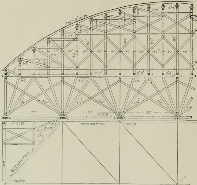
Fig. 3.—Details of Timber Center for 281-Foot Concrete Arch, Spokane, Washington
