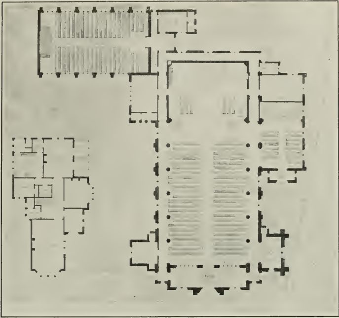
Floor Plan of St. Paul's Church and Rectory, Oakland, California Ben G. McDougall, Architect
