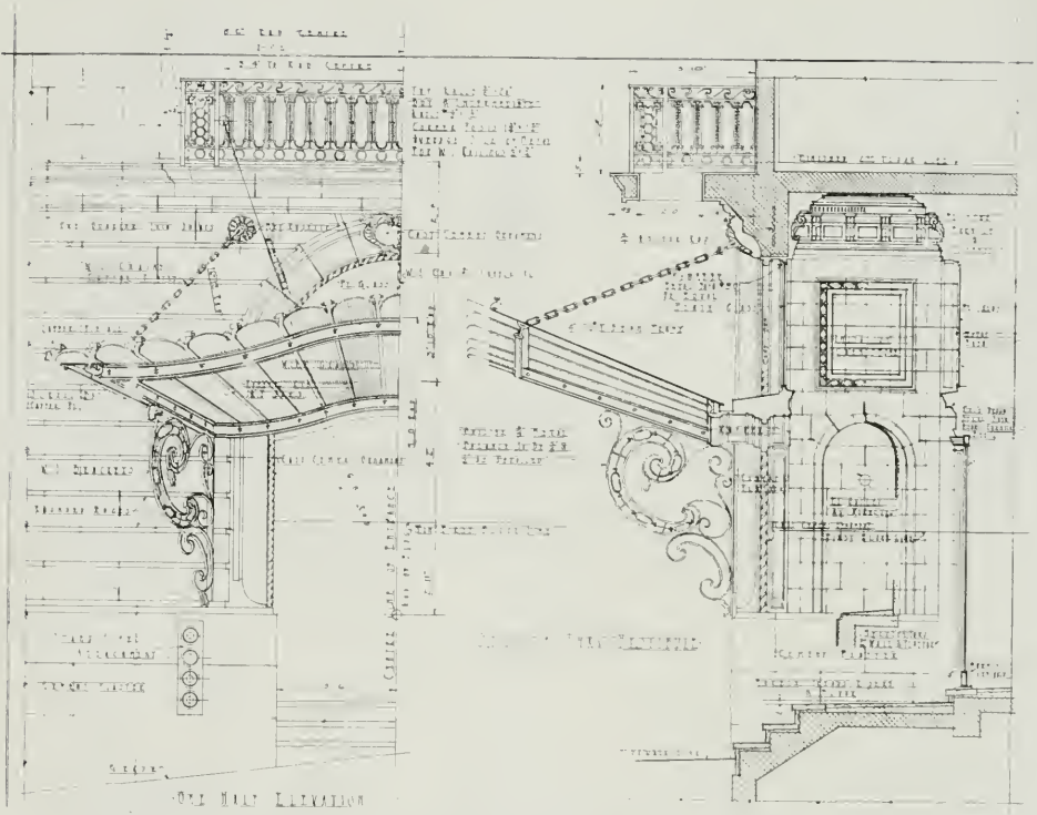
DETAILS, APARTMENT HOUSE FOR MR. A. W. WILSON, SAN FRANCISCO C. A. Meussdorffer, Architect
