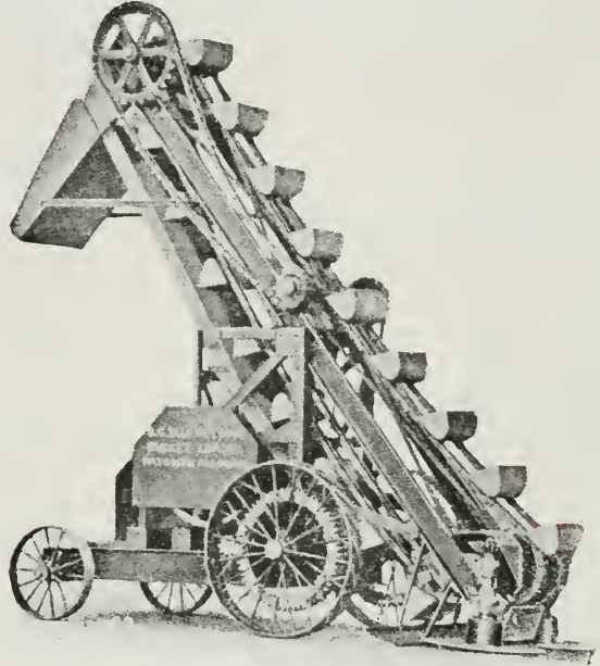
B-G SELF FEEDING LOADER
