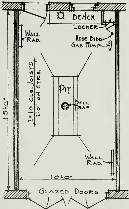
-TYPICAL- PLAN- Scale 0 1 2 3 4 5 6 7 8 9 10 feet
