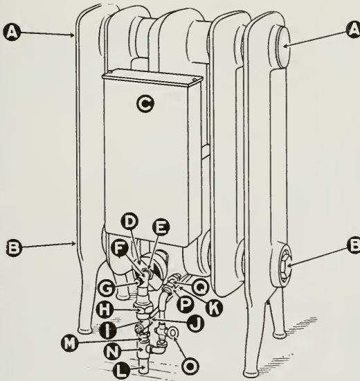
No. 1—Five Sections REAR VIEW, showing how to make connection, and where burner is regulated. A—Safety Valves E—Lock Nut I—Stop Cock B—Plugs F—Needle Valve J—Set Screw C—Retort G—Needle Cap Screw K—Valve Stem D—Air Shutter H—Union L—Gas Supply Pipe (Above connections are \frac{3}{8} inch pipe) If pilot light is to be connected use M—Close Nipple O—Pilot Stop Cock Q—Pilot Connection N—Tee ( \frac{3}{8} x \frac{3}{8} x \frac{1}{8} ) P—Pilot Union (Pilot line \frac{1}{8} in. pipe)
