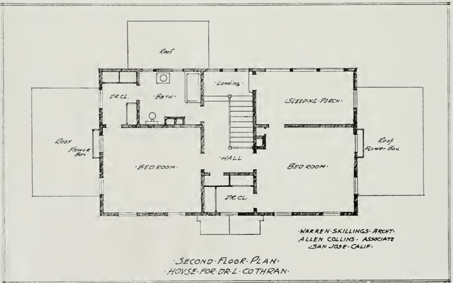
SECOND FLOOR PLAN, HOUSE FOR DR. LINCOLN COTHRAN, SAN JOSE Warren Skillings, Architect
