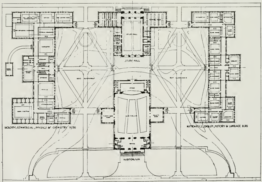
COMPETITION FOR FULLERTON UNION HIGH SCHOOL AND JUNIOR COLLEGE FIRST FLOOR PLAN, PLACED FOURTH ELMER GREY, ARCHITECT
