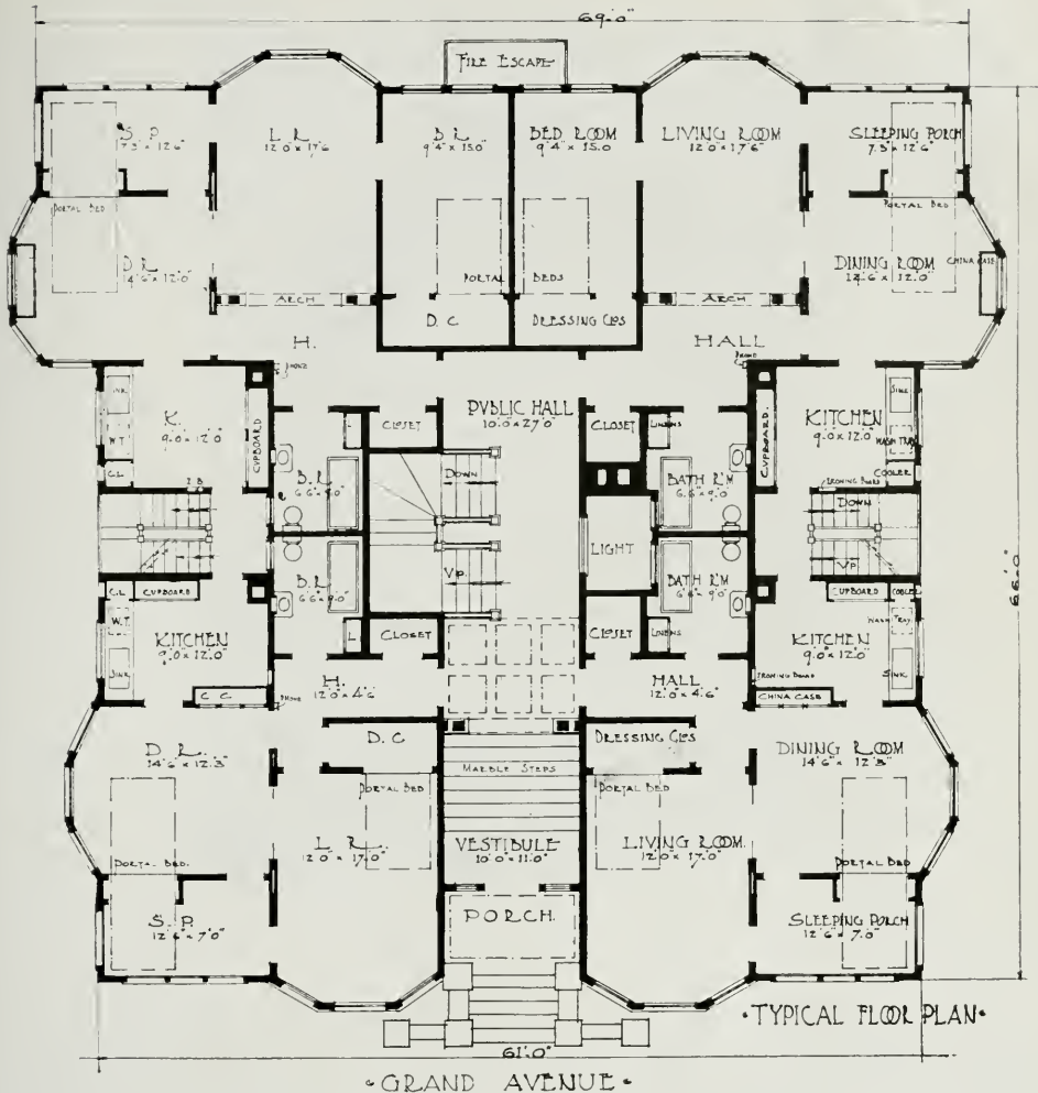
PLAN, LENNOX APARTMENTS, OAKLAND
