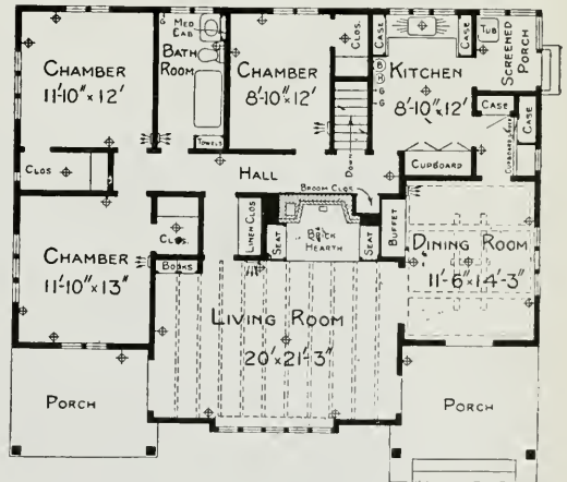
Floor Plan of House Indicated on Lot No. 11—Scale \frac{1}{16} In. to the Foot.
