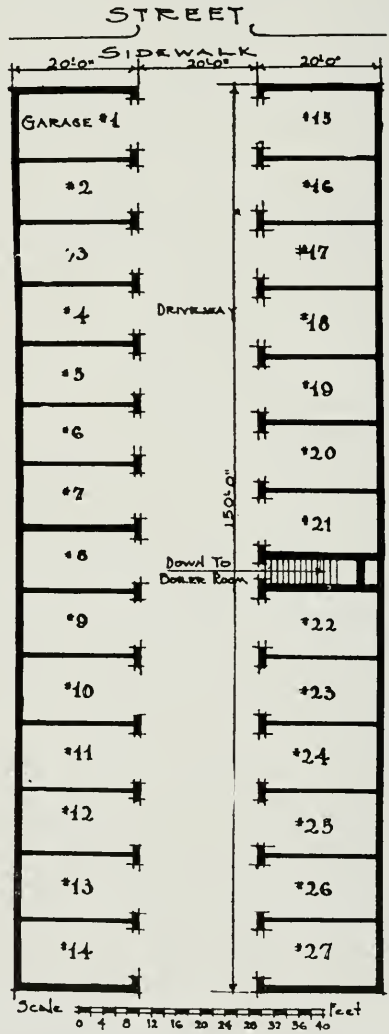
No. 2.—A plan for a lot of 150 feet deep by sixty feet wide. Where the units are built with the rear wall on the property line, it will usually be necessary to use small skylights to obtain light.
