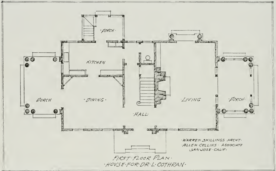
FIRST FLOOR PLAN, HOUSE FOR DR. LINCOLN COTHRAN, SAN JOSE Warren Skillings, Architect
