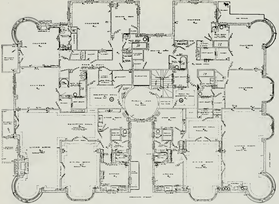
5 TH STORY FLOOR PLAN SCALE 1/8" = 1'-0" TYPICAL FLOOR PLAN, SUMMIT APARTMENTS, SAN FRANCISCO T. Paterson Ross, Architect
