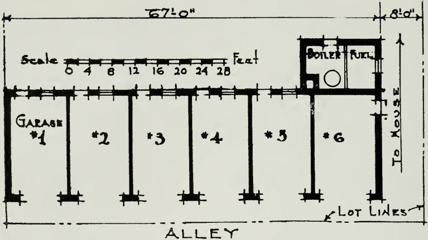
GARAGE SHED FOR APARTMENT HOUSE No. 3.—This plan is suitable for rear portion of a wide lot.
