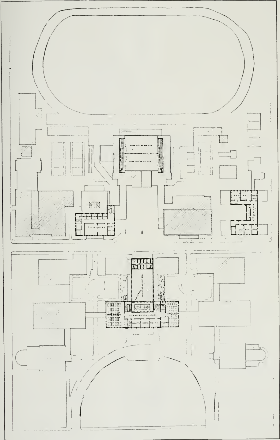
COMPETITION FOR BULLERTON UNION HIGH SCHOOL AND JUNIOR COLLEGE SECOND FLOOR PLAN, PLACED THIRD ALLISON & ALLISON, ARCHITECTS
