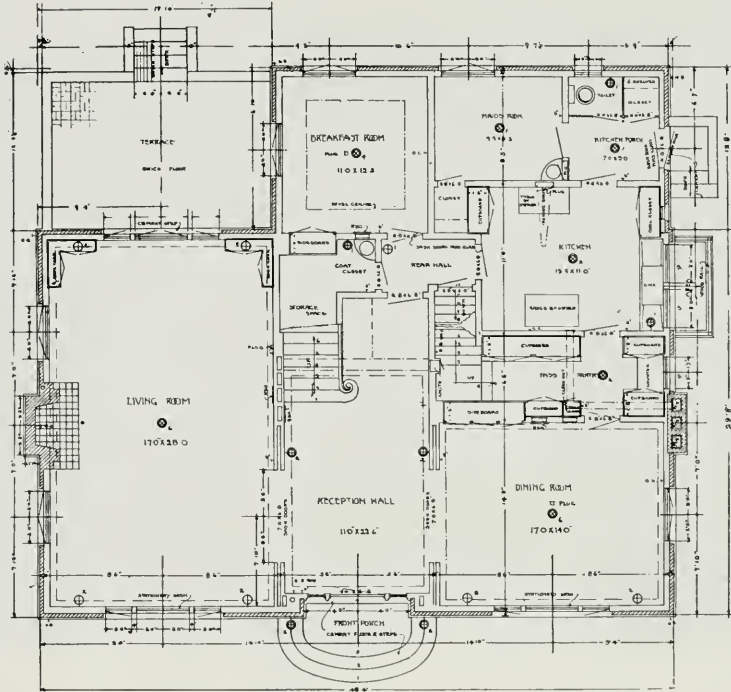
FIRST FLOOR PLAN, HOUSE OF MR. E. B. DAVIS, BERKELEY
