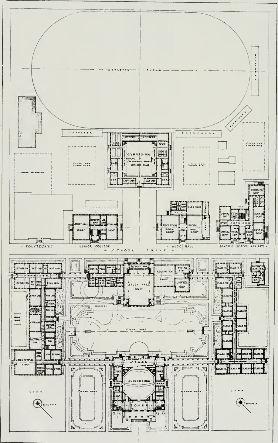
COMPETITION FOR FULLERTON UNION HIGH SCHOOL AND JUNIOR COLLEGE FIRST FLOOR PLAN, PLACED MOTT E. MARSTON, ARCHITECT
