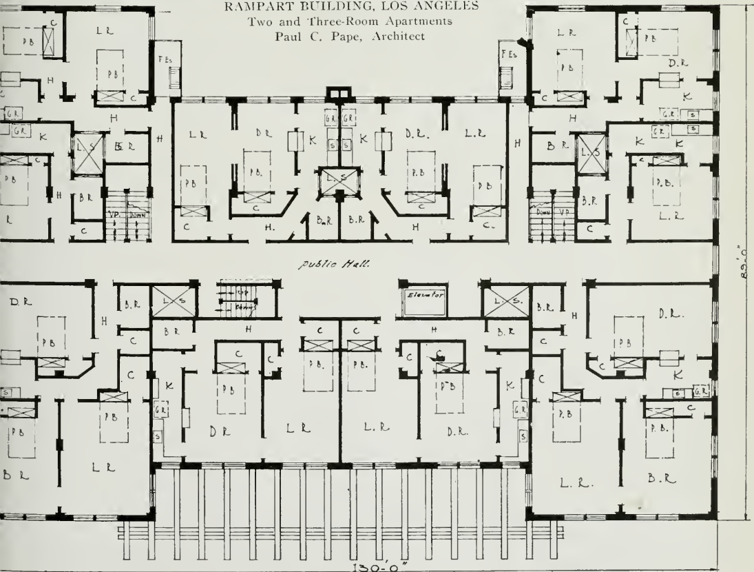
TYPICAL FLOOR PLAN, RAMPART APARTMENTS, LOS ANGELES
