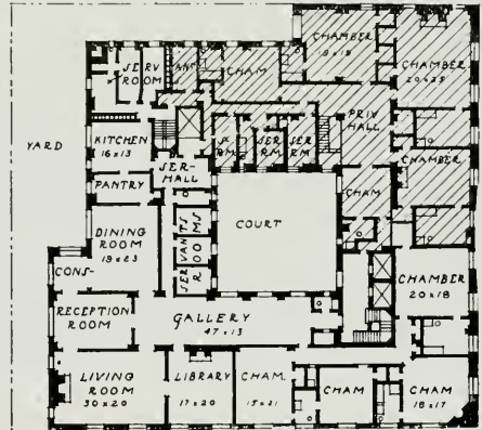
SIXTH, EIGHTH AND TENTH FLOOR PLANS, SHOWING DUPLEX TYPE APARTMENT BUILDING, 907 FIFTH AVE., NEW YORK CITY J. E. R. Carpenter, Architect
