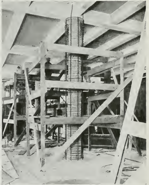
Fig. 2.—Showing additional reinforcing steel in place and ready for new form work.
