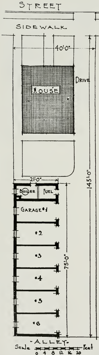
No. 1.—This plan is suitable for a comparatively narrow lot. In a scheme of this sort the entrance from the street is often omitted, the only entrance being from the alley in the rear of the lot.
