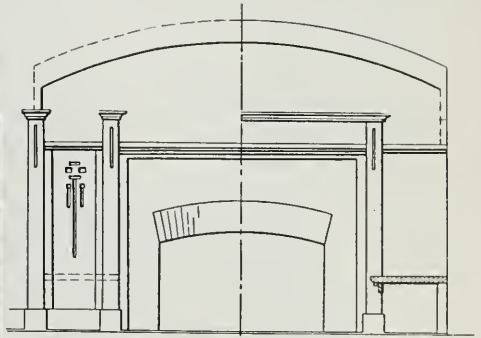
The Living Room Angle Nook—Scale \frac{1}{4} In. to the Foot
