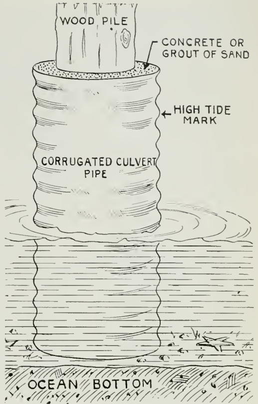
How wooden piles can be protected from the attacks of the Teredo by means of Armco Iron Casings.
