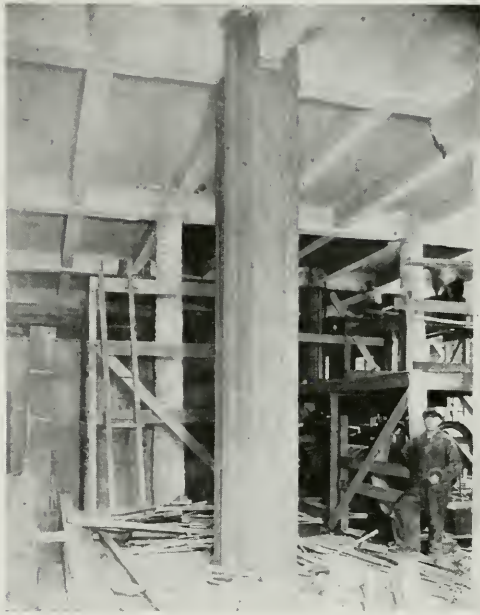
Fig. 3.—Showing finished column after removal of forms. Concrete was poured from floor above through holes cut in floor slab.
