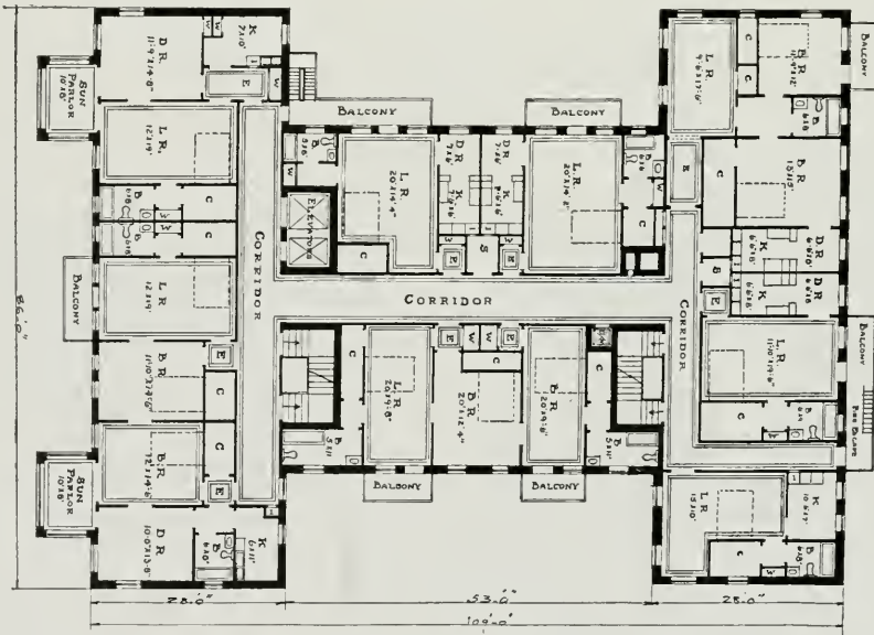
TYPICAL FLOOR PLAN, CLIFTON APARTMENTS, NASHVILLE, TENN. All Two and Three-Room Apartments.
