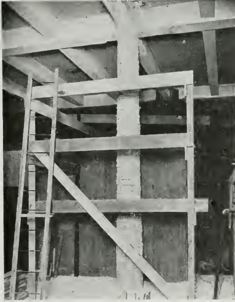
Fig. 1.—Showing fireproofing removed from existing column in Oceanic building, San Francisco, and ready to receive additional reinforcing steel to support three extra floors.
