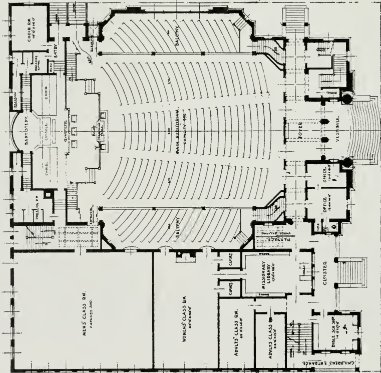
MAIN FLOOR PLAN FIRST CHRISTIAN CHURCH, LONG BEACH, CALIF. ARCHITECT: R. O. COLE, ARCHITECT 254 S. 7TH ST. LOS ANGELES, CALIF.
