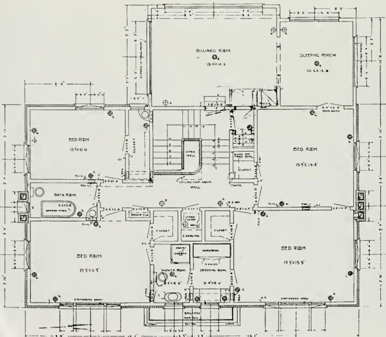
SECOND FLOOR PLAN, HOUSE OF MR. E. B. DAVIS, BERKELEY Sidney B. Newsom, Architect
