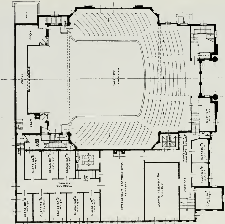
GALLERY FLOOR PLAN FIRST CHRISTIAN CHURCH, LONG BEACH, CALIF. ARCHITECT: R. O. COLE, ARCHITECT 254 S. 7TH ST. LOS ANGELES, CALIF.
