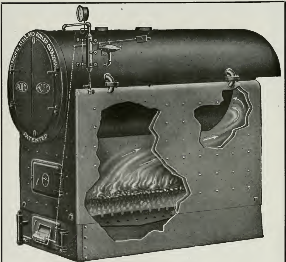
PACIFIC DOUBLE RETURN FIRE BOX STEAM BOILER
