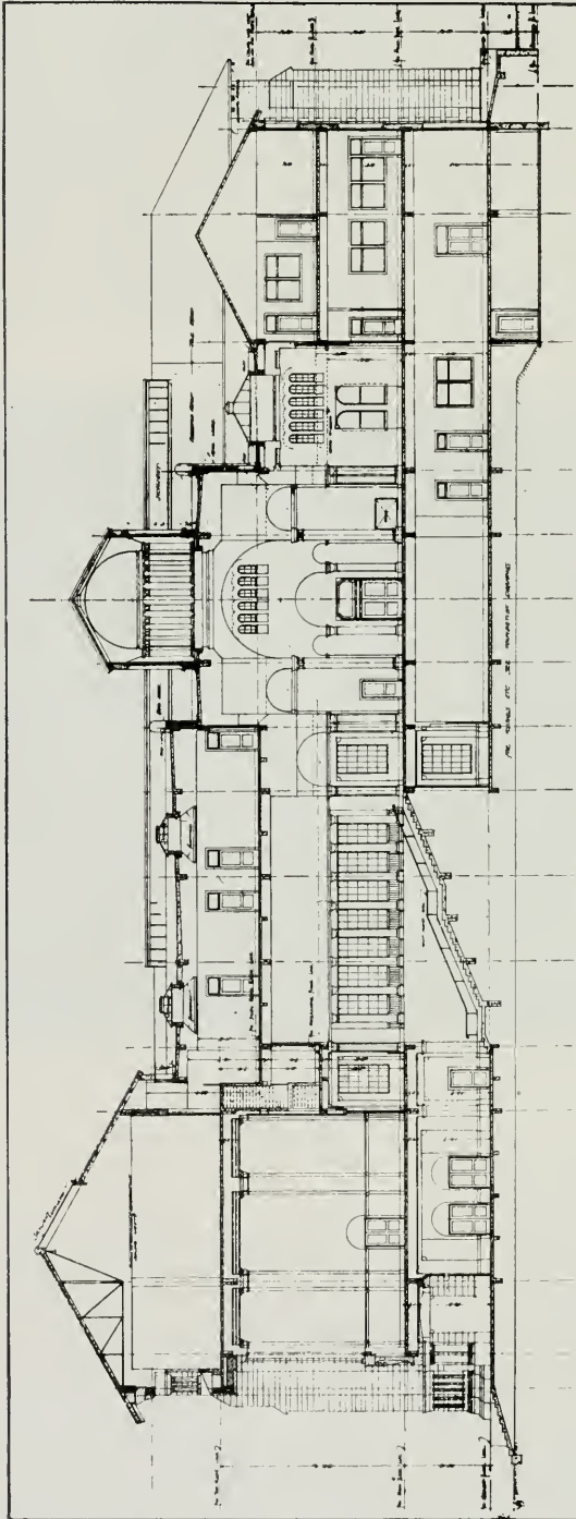
LONGITUDINAL SECTION OF LIBRARY LELAND STANFORD JR. UNIVERSITY BAKEWELL & BROWN, ARCHITECTS
