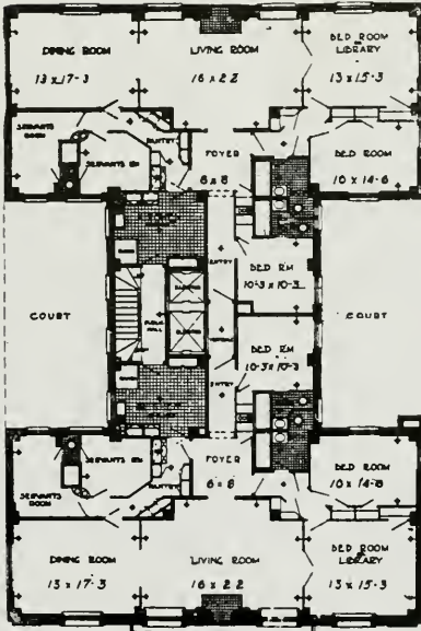
TYPICAL FLOOR PLAN 116 EAST FIFTY-EIGHTH ST., NEW YORK CITY J. E. R. Carpenter, Architect
