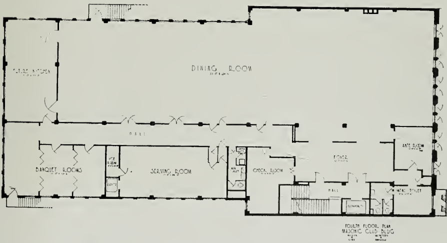
FOURTH FLOOR PLAN, MASONIC CLUB BUILDING, LOS ANGELES Walker and Eisen, Architects and Engineers
