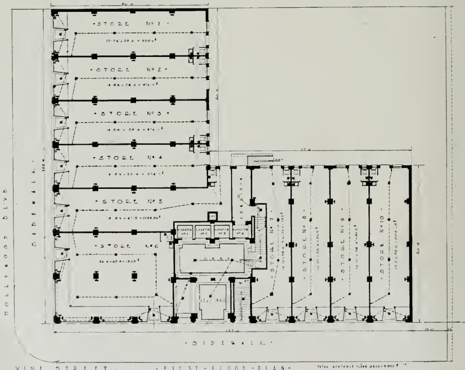
VIN STREET - FIRST FLOOR PLAN - FIRST FLOOR PLAN, TAFT BUILDING, HOLLYWOOD Walker and Eisen, Architects and Engineers
