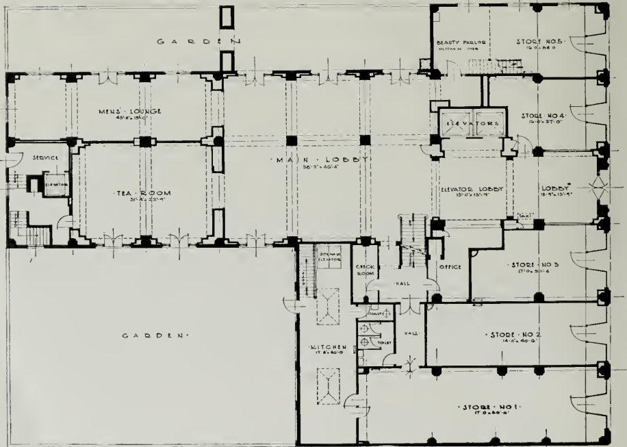
PLANS, HOLLYWOOD PLAZA HOTEL, HOLLYWOOD Walker and Eisen, Architects and Engineers
