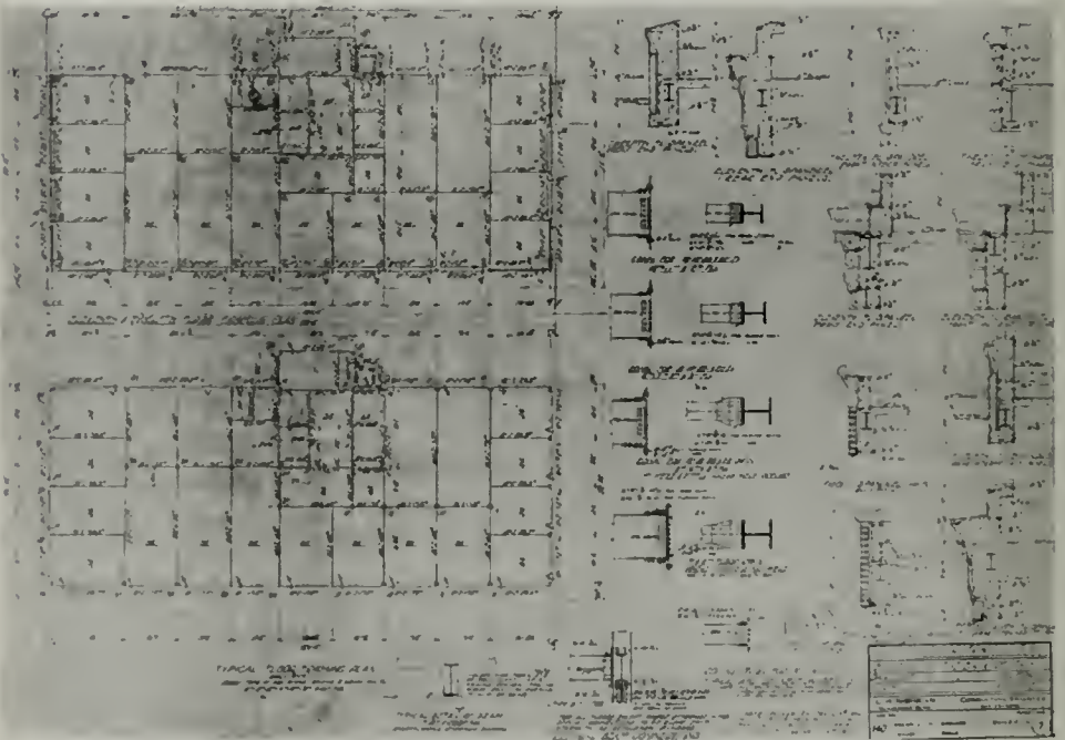
TYPICAL FLOOR FRAMING PLAN, BANK OF ITALY, SAN JOSE L. H. Nishkian, Structural Engineer
