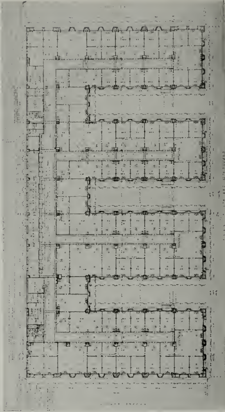
TYPICAL PLAN, DEXTER HORTON BUILDING, SEATTLE ARCHITECT AND ENGINEER JOHN GRAHAM,
