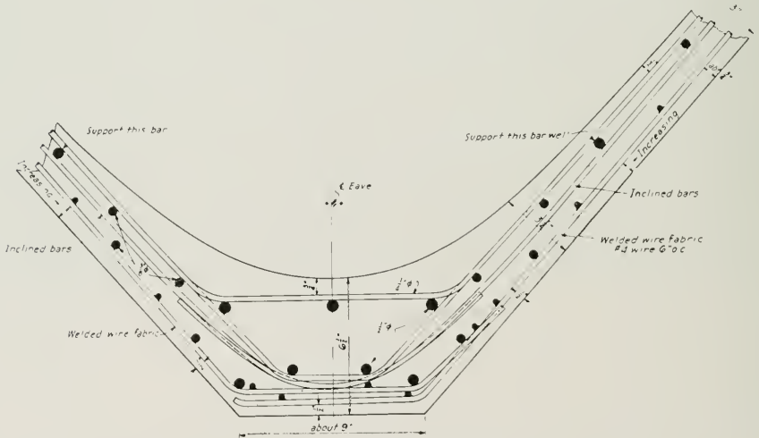
DETAIL SECTION THROUGH VALLEY
