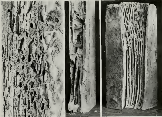
Fig. 27.—Workings of the ground dwelling termites. All show the earthy frass characteristic of the subterranean termites. The tendency to select the soft portion of the annual rings is shown in b in coarse grained wood, and in c in close grained wood. In both cases the work was wholly internal, without external evidences of its existence except at the ends of the members. Pieces a and c were sound wood without visible evidence of fungus attack.
