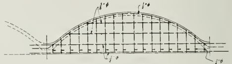
SECTION OF TYPICAL END FRAMES (GABLES) WITHOUT WINDOWS (FRONT WALL)
