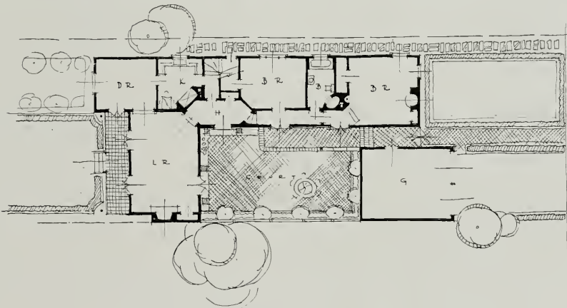
PLAN, HOUSE OF MR. AND MRS. M. C. WANTZ, BERKELEY Frederick L. Confer, Architect
