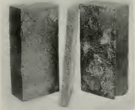
Figure 1—Poor bond distribution obtained with unadaptable mortar. Dry porous bricks laid with portland cement mortar deficient in water retaining capacity.
