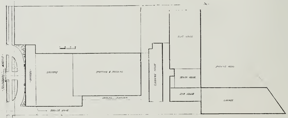
PLOT PLAN, MARSHALL STEEL PLANT, OAKLAND Alben Froberg, Architect
