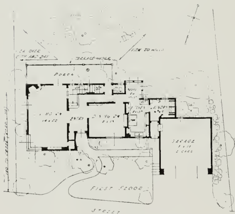
FIRST FLOOR PLAN, HOUSE OF MR. AND MRS. HERMAN BISHOPRIC, PIEDMONT, CALIFORNIA W. R. Yelland, Architect
