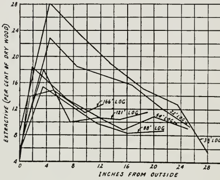
FIG. 1—DISTRIBUTION OF EXTRACTIVE IN REDWOOD. CHART BY SHERRARD AND KURTH.
