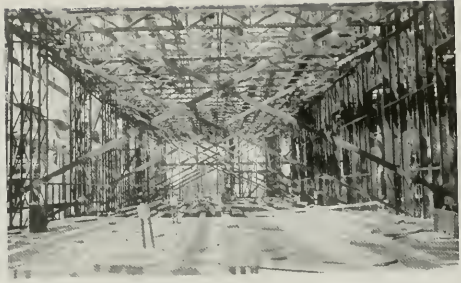
EARTHQUAKE BRACING IN ALL NON-BEARING TRANSVERSE PARTITIONS
