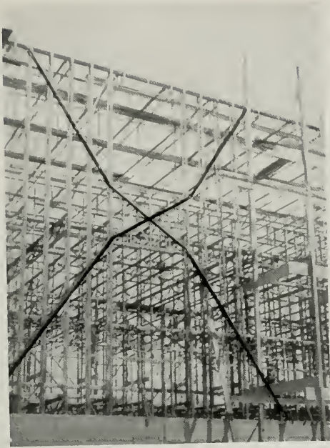
EARTHQUAKE BRACING ON LOAD BEARING WALLS
