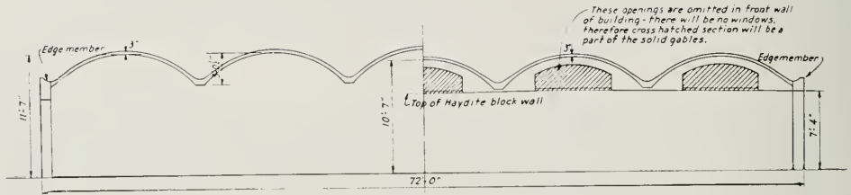
TRANSVERSE SECTION
