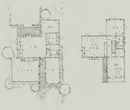
PLANS, HOUSE OF MR. AND MRS. RAYMOND BOWERS, BERKELEY Frederick L. Confer, Architect
