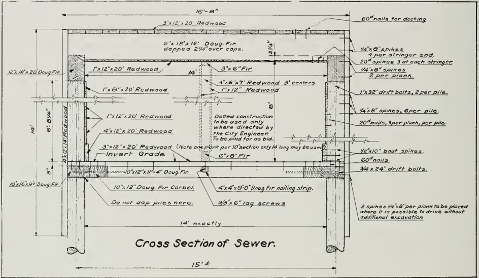
FIG. 1—CROSS SECTION OF ISLAIS CREEK SEWER, SAN FRANCISCO
