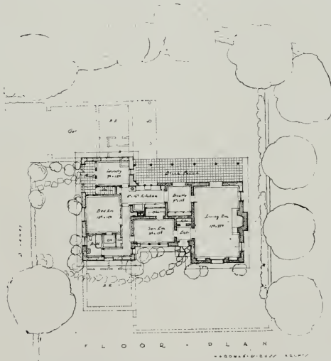
PLAN, ADOBE HOUSE FOR HARRY HINDMAN, LAFAYETTE, CALIFORNIA Hardman & Russ, Architects
