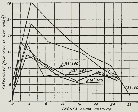
FIG. 3—DISTRIBUTION OF HOT-WATER-SOLUBLE EXTRACTIVE IN A VIRGIN REDWOOD TREE THROUGHOUT CROSS SECTIONS TAKEN FROM SIX HEIGHTS. CHART PREPARED BY SHERRARD AND KURTH OF FOREST PRODUCTS LABORATORY, FOREST SERVICE, U. S. DEPT. OF AGRICULTURE, MADISON, WISCONSIN.
