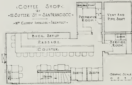
PLAN, COFFEE SHOP, 111 SUTTER STREET, SAN FRANCISCO Wm. Clement Ambrose, Architect
