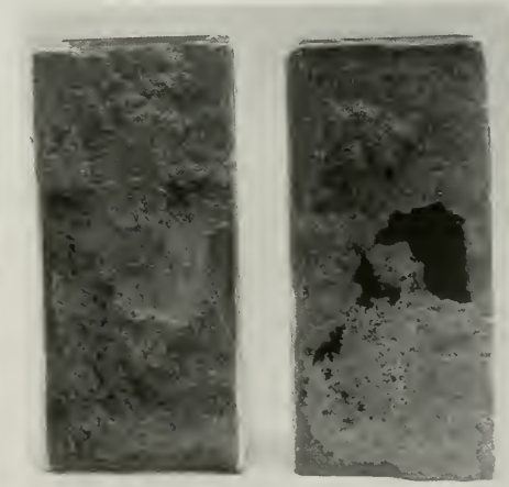
Figure 3—Same bricks, same mortar as illustrated in Figures 1 and 2. In this case, the bricks were almost completely saturated (too wet) when laid. Figures 1, 2 and 3 illustrate the fact that given a poorly adaptable mortar, wetting bricks does not solve the problem of getting good extent of bond.
