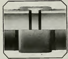
Section of National DUROLINE Pipe coupling and joint. (Note special highly corrosion-resistant joint compound on end of pipe and on threads.)
