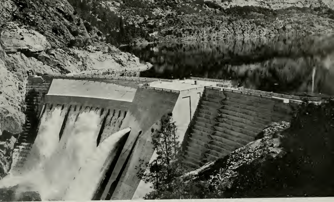
O'SHAUGHNESSY DAM ON TUOLUMNE RIVER IN YOSEMITE NATIONAL PARK The dam has a total height of 344 feet which will be increased to 430 feet at a cost of $3,500,000. The present dam was completed in 1923 at a cost of $7,000,000.
