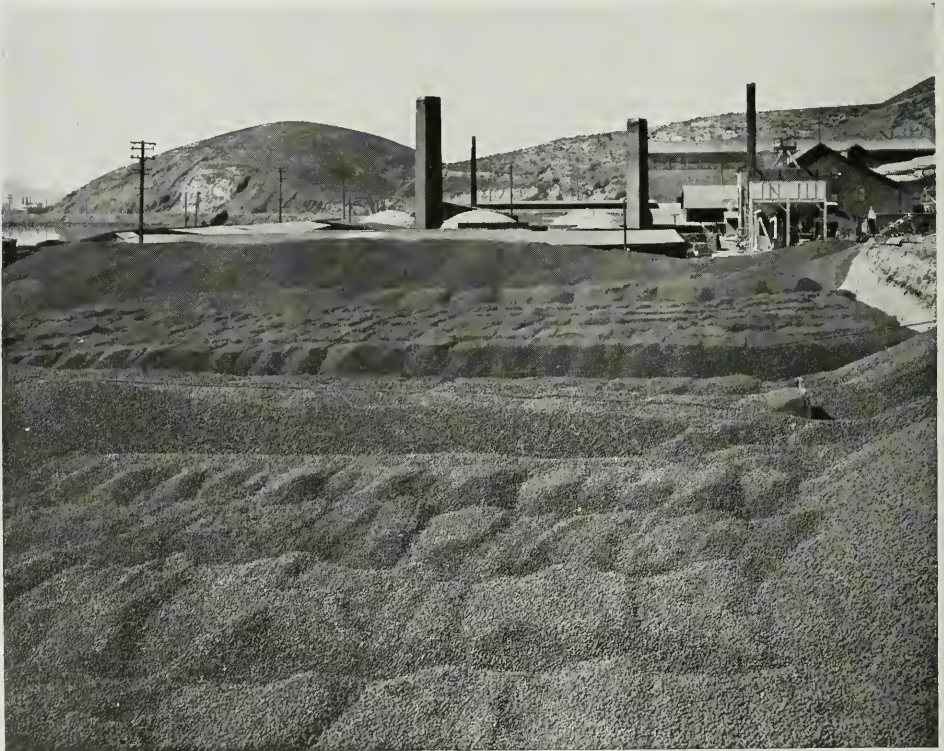
STOCK PILE OF GRAVELITE AT PLANT, POINT RICHMOND, CALIFORNIA This material mixed with cement makes a light weight concrete that is destined to revolutionize the present method of making structural concrete. Engineers say its use on the upper deck of the Bay Bridge will mean a saving of 20,000 tons in dead weight
