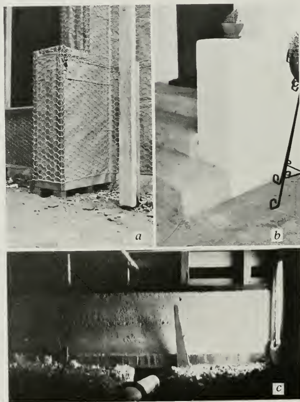
Fig. 3— a —before, b —after completion. The wood frame of buttress wall is in contact with the soil, lacking a proper foundation. The earth fill supporting the concrete steps is banked against the wood frame of the house below the entrance and against the side of the buttresses providing conditions favoring rapid destruction of timber by decay and termite attack. ( c )—Form board left in place along interior of foundation wall. Wood forms buried in the soil provide breeding places for subterranean termites.
