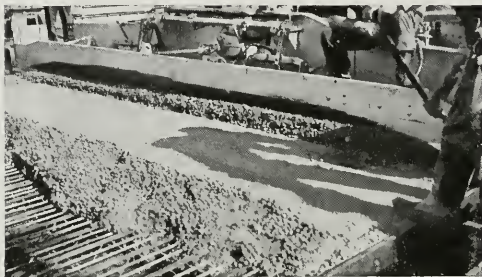
CLOSE-UP, SHOWING VIBRATING SCREEN IN OPERATION AND STEEL REINFORCEMENT
