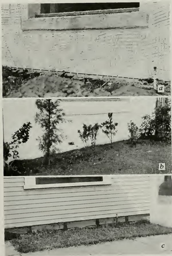
Fig. 4—Conditions at the foundation which invite attack by subterranean termites. (a)—Foundation wall too low. Dotted line is just above the top of the sill which rests on the foundation wall. (b)—Same house as in (a), after the top-soil had been placed and planting completed the grade level was above the sill. (c)—The ends of 2 inch by 12 inch floor joists as shown rest on concrete foundation wall, the top of wall being 9 inches below the grade level of the soil. The ends of the joists were so badly damaged that they had practically no bearing on the foundation wall.
