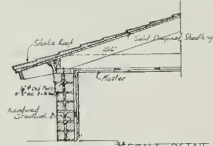
SCALE-DETAIL EXTERIOR WALL AT EAVES
