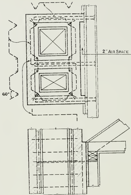
SKETCH SHOWING METHOD OF CONSTRUCTING REINFORCED BRICK CHIMNEY
