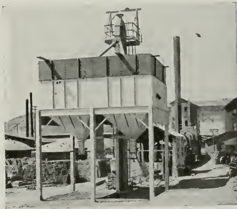
ROTARY KILN AND HOT STORAGE BIN AT GRAVELITE PLANT, POINT RICHMOND
