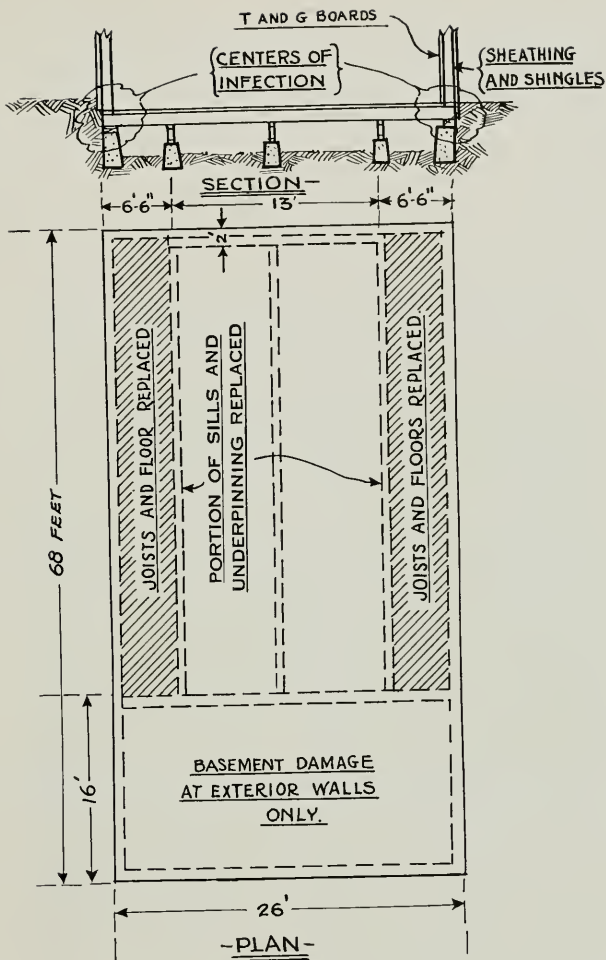
Fig. 2—Plan of building seriously damaged by damp-wood termite. Earth in contact with the wood frame is a source of infestation.
