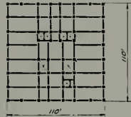
PLAN AT 7TH FLOOR STEEL
