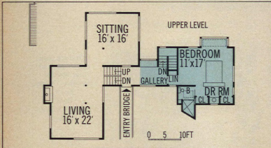
Floor plan of house's upper level (above) shows new bedroom wing (shaded area) at the end of a connecting gallery. Addition has 700 square feet, including laundry/dressing area below. House's lower level contains kitchen and a guest room formerly the master bedroom. Broken lines in bath and window bay indicate skylights.
