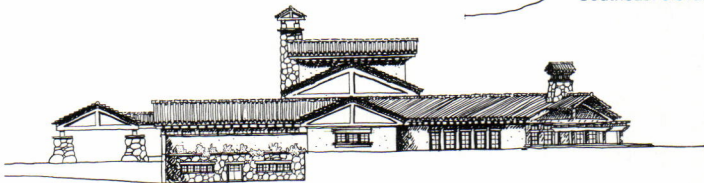
Northeast elevation
