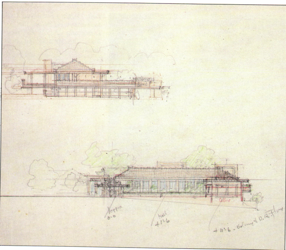
Above left, two elevations of the Goto house, color pencil and graphite pencil on tracing paper dated May 1921. Above, preliminary sketch of the Immu house, 1918.
