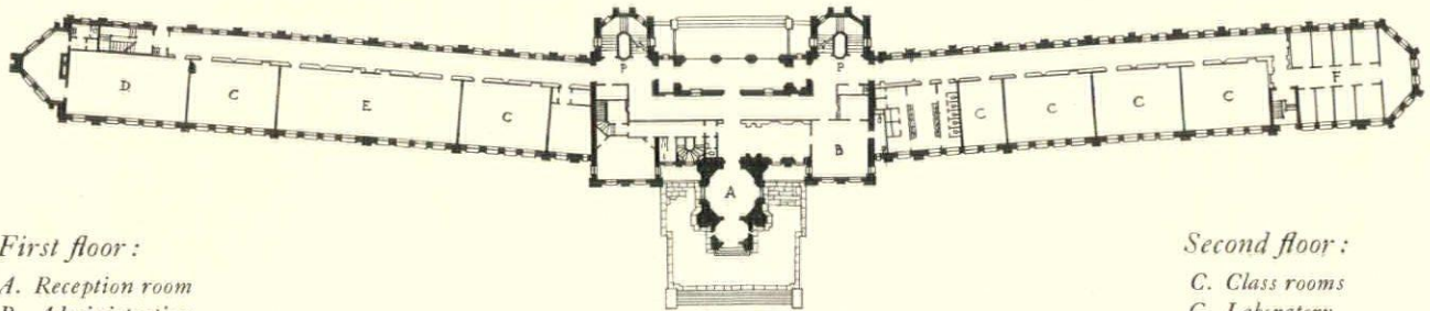
First-floor plan
