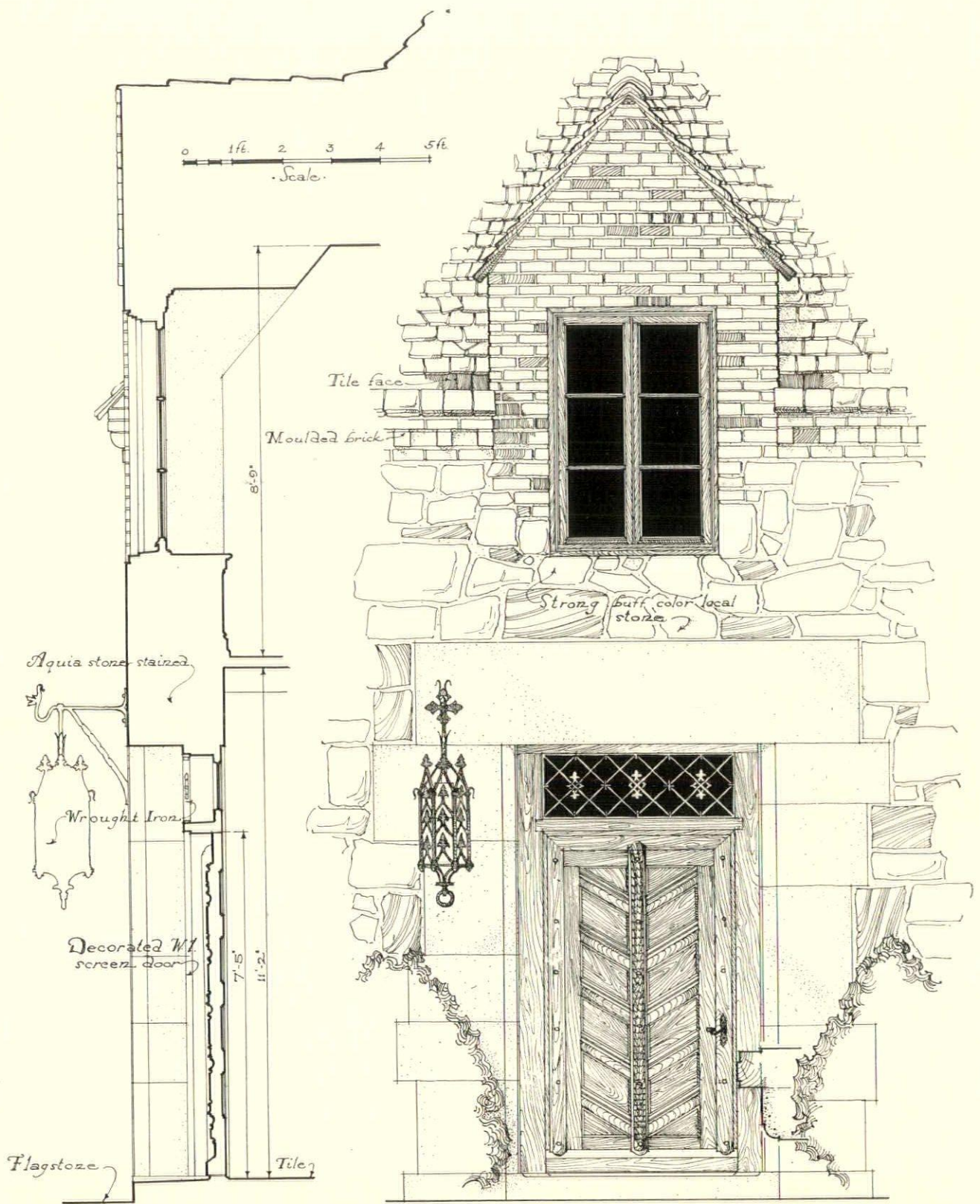
Section
