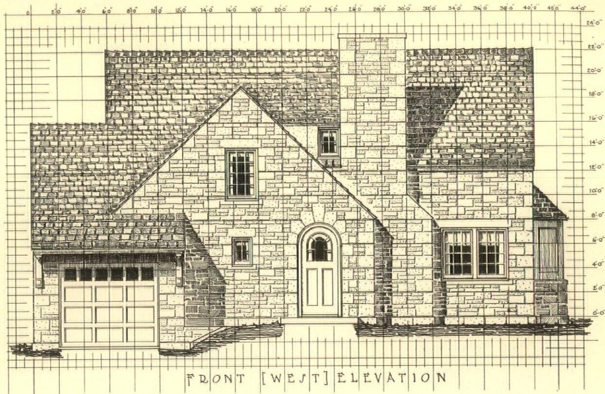
Front elevation, on which is superimposed the modular scale with the squares representing 4", reproduced at a scale of \frac{1}{8} " to the foot
