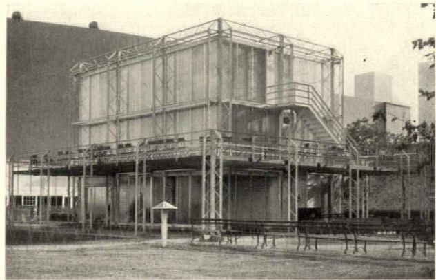
A house at the Chicago Fair with steel supports outside. George Fred Keck, architect
