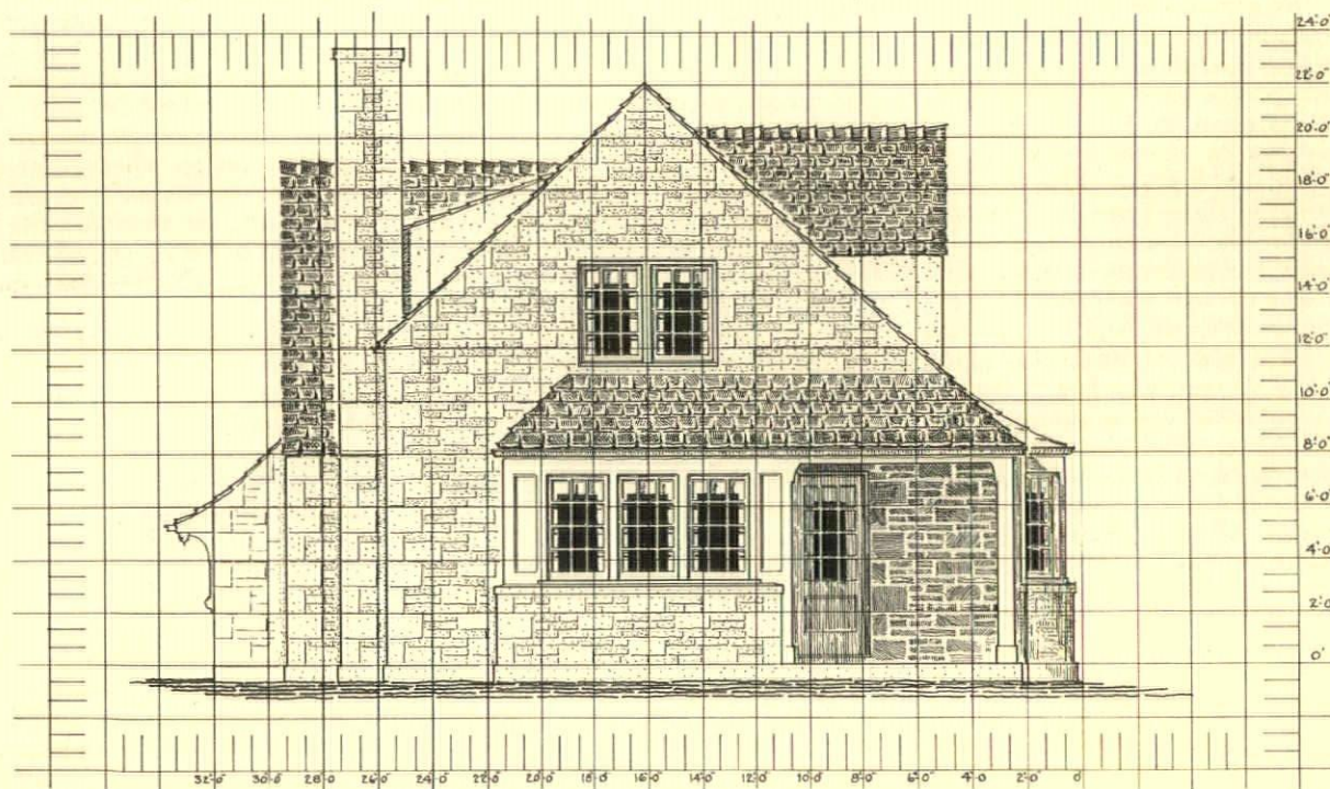
END [SOUTH] ELEVATION
