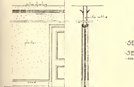
ELEVATION SECTION TYPE "D"
