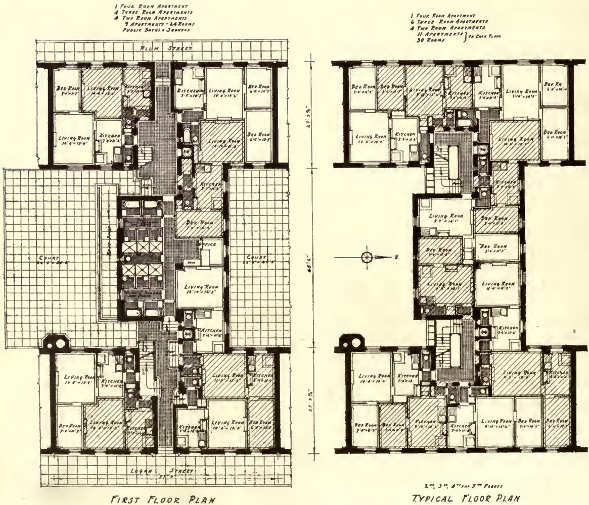
FIGURE V—MODEL FIREPROOF TENEMENT AT CINCINNATI, OHIO
