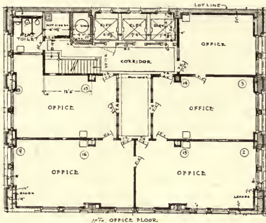
16TH OFFICE FLOOR
