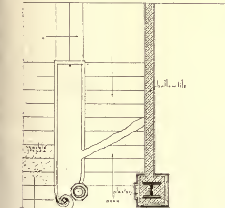
HALF PLAN TYPICAL STAIRCASE
