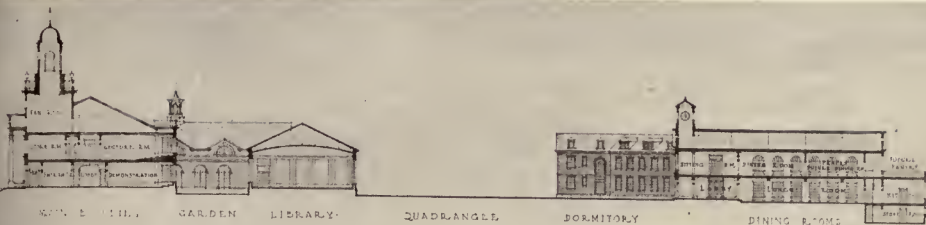
- SECTIONS - SCALE 1/32" = 1'-0"
