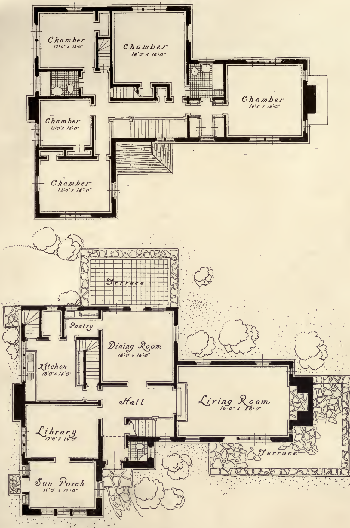
HOUSE OF CLARENCE McDANIEL, HARTSDALE, NEW YORK JULIUS GREGORY, ARCHITECT
