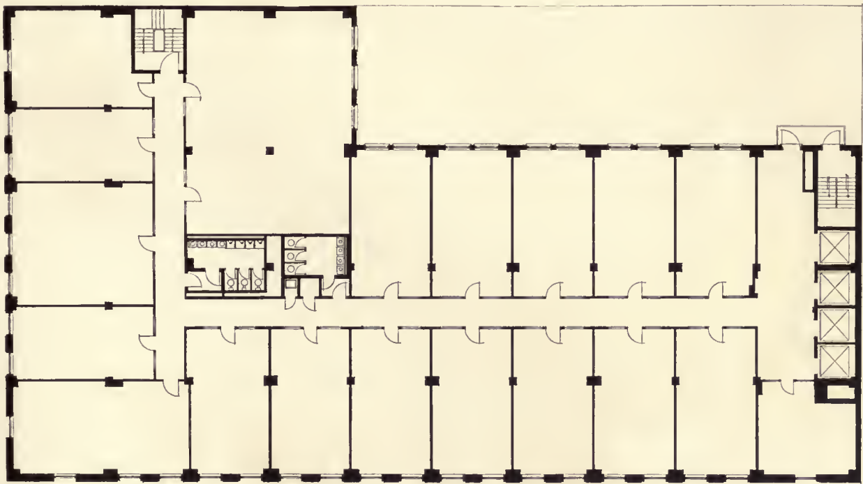
TYPICAL FLOOR PLAN BUILDING FOR S. W. STRAUS & CO., FIFTH AVENUE AT 46TH STREET, NEW YORK WARREN & WETMORE, ARCHITECTS
