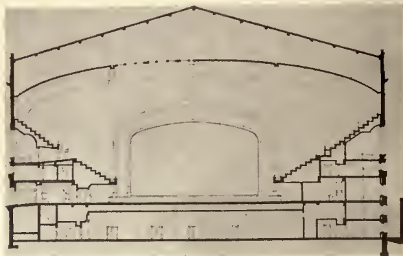
CROSS SECTION LOOKING TOWARDS THE STAGE
