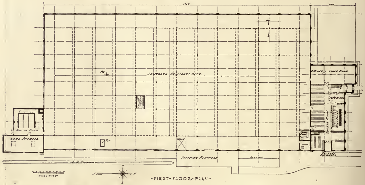
BUILDING FOR WALKER VEHICLE CO., CHICAGO, ILL. GEORGE C. NIMMONS & CO., ARCHITECTS.
