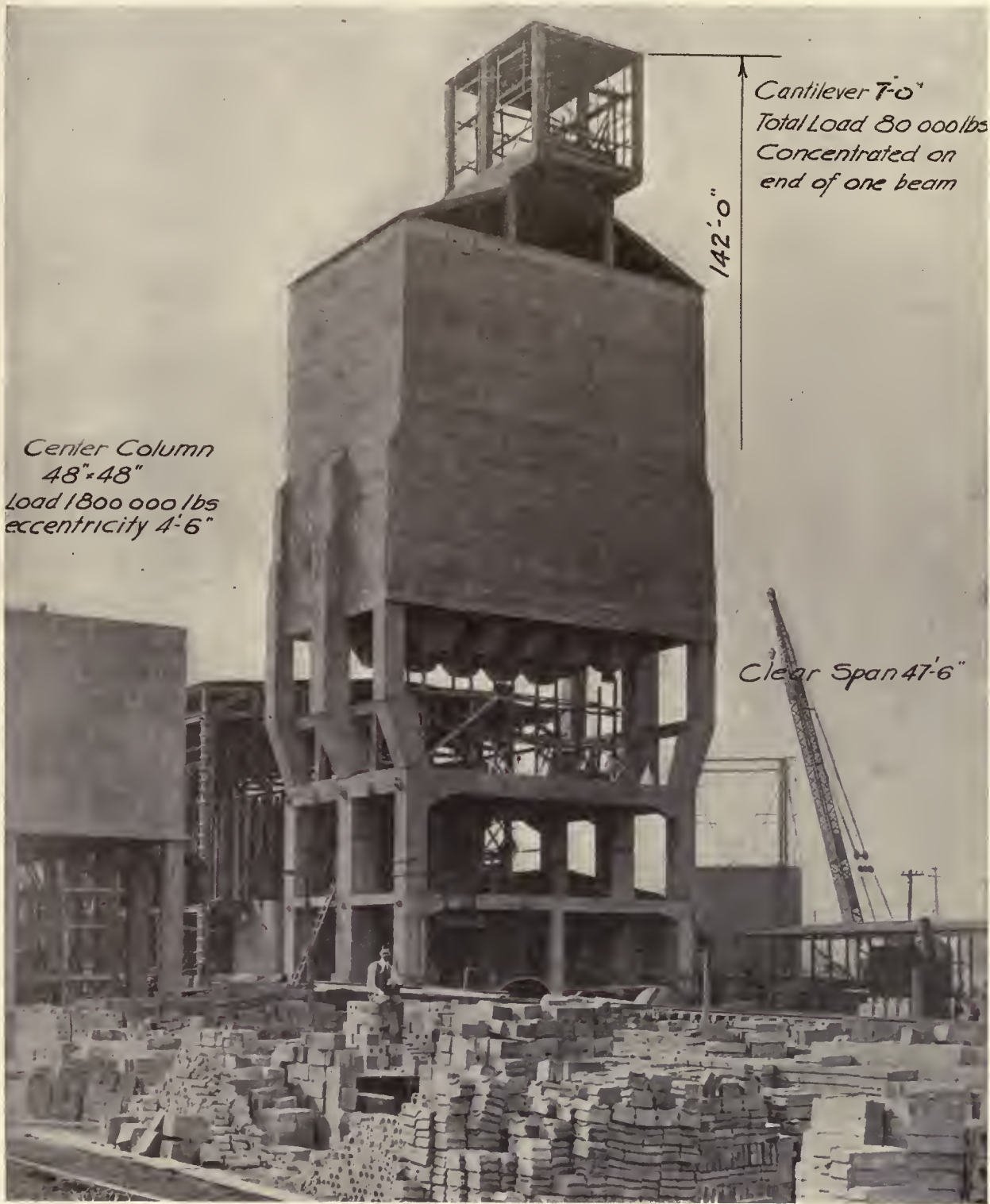
COAL BIN FOR ST. LOUIS COKE & CHEMICAL CO., GRANITE CITY, ILL. L. J. MENSCH, ENGINEER
