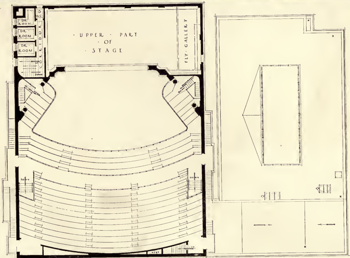
VIEW LOOKING ACROSS BALCONY AND BALCONY FLOOR PLAN BROADWAY THEATRE, SOUTH BOSTON, MASS. BLACKALL, CLAPP & WHITEMORE, ARCHITECTS
