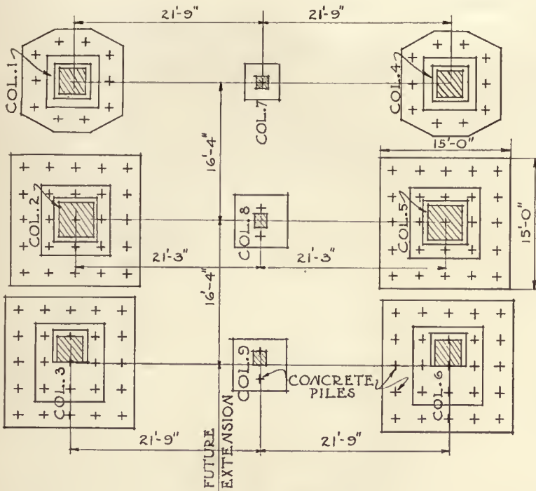
SECTION A-A. FOOTING PLAN
