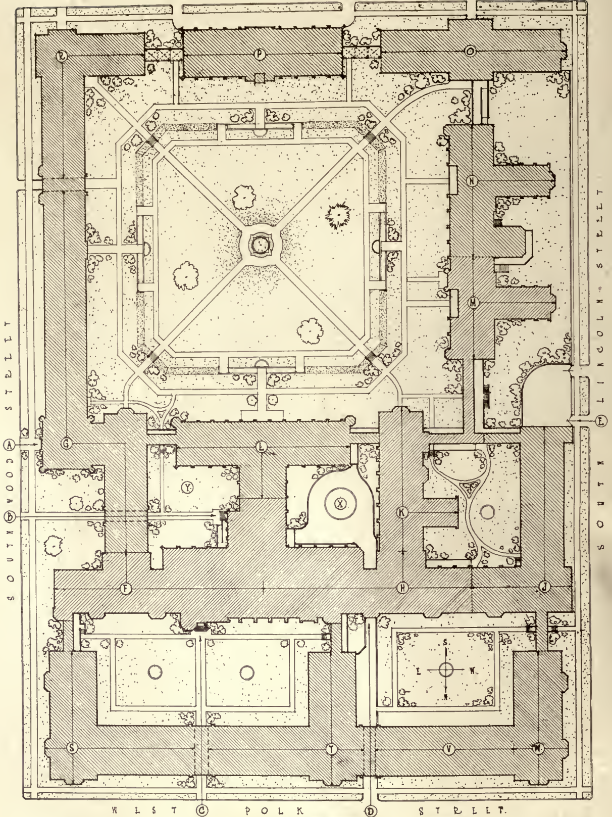
* RESEARCH & EDUCATIONAL HOSPITALS OF THE STATE OF ILLINOIS * - EDGAR MARTIN, SUPERVISING ARCHITECT - RICHARD L. SCHMIDT, GARDEN & MARTIN ASSOCIATE ARCHITECTS - BUILDINGS NOW UNDER CONSTRUCTION. [Hatched Area] SCALE 100 FEET. FUTURE DEVELOPMENT [Dotted Area] (A) ADMINISTRATION ENTRANCE (B) OUT PATIENTS ENTRANCE (C) STUDENTS & NURSES ENTRANCE (D) AMBULANCE ENTRANCE (E) KITCHEN ENTRANCE (F) CLINICAL INSTITUTE (G) EXTENSION OF CLINICAL INSTITUTE (H) EYE & EAR INFIRMARY (I) EXTENSION OF EYE & EAR INFIRMARY (J) PSYCHIATRIC INSTITUTE (K) ADMINISTRATION BUILDING (L) ORTHOPEDIC INSTITUTE (M) EXTENSION OF ORTHOPEDIC INSTITUTE (N) INFECTIOUS DISEASES (O) POWER PLANT (P) VENEREAL DISEASES (Q) RESEARCH INSTITUTE (R) LIBRARY CLASS ROOMS & RESEARCH LABORATORIES (S) CLASS ROOMS & LABORATORIES (T) DENTAL INSTITUTE (U) AMBULANCE COURT (V) DISPENSARY COURT 5/3/1920
