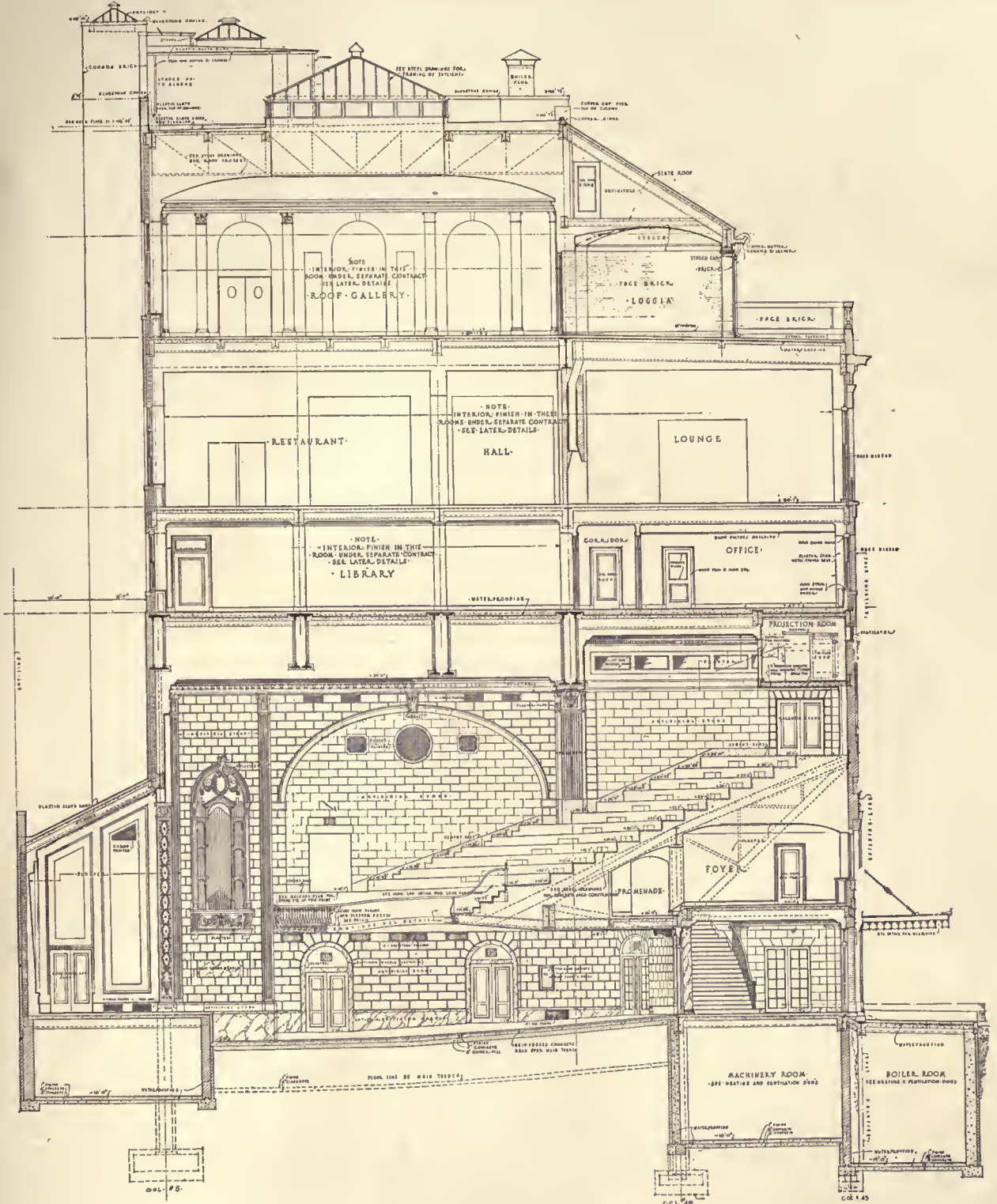
LONGITUDINAL SECTION THE TOWN HALL, NEW YORK CITY MCKIM, MEAD & WHITE, ARCHITECTS
