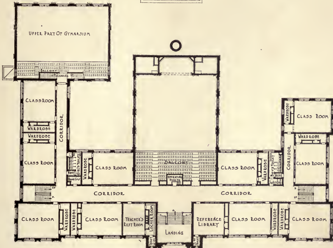
SECOND FLOOR AND ROOF PLANS DELAWARE SCHOOL, SYRACUSE, NEW YORK JAMES A. RANDALL, ARCHITECT
