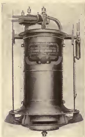
FIG. 11. ONE TYPE OF ATOMIZING HUMIDIFIER TO BE PLACED IN ROOM WHERE MOISTURE IS DESIRED
