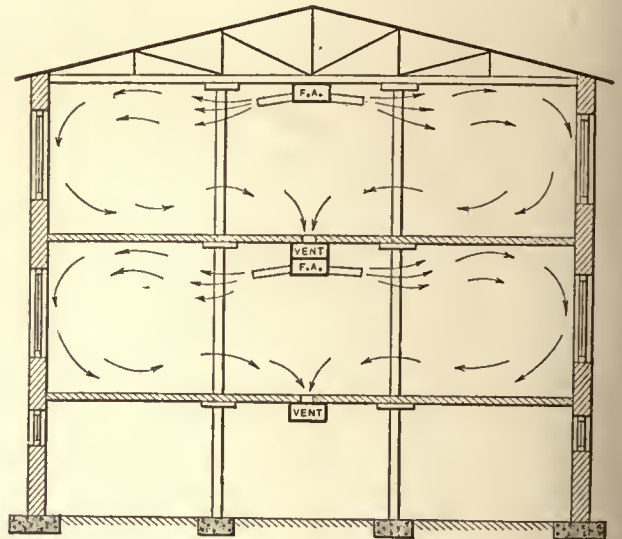
FIG. 4. ANOTHER ARRANGEMENT FOR BUILDINGS SEVERAL STORIES HIGH
