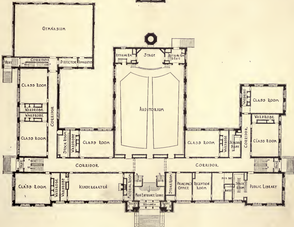
BASEMENT AND FIRST FLOOR PLANS DELAWARE SCHOOL, SYRACUSE, NEW YORK JAMES A. RANDALL, ARCHITECT
