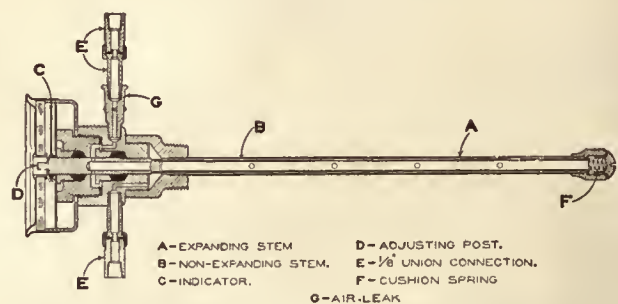
FIG. 3. SECTION SHOWING CONSTRUCTION OF AN INSERTION THERMOSTAT
