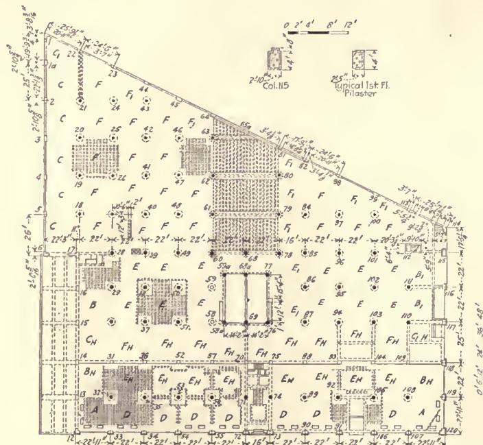
FLOOR PLAN
