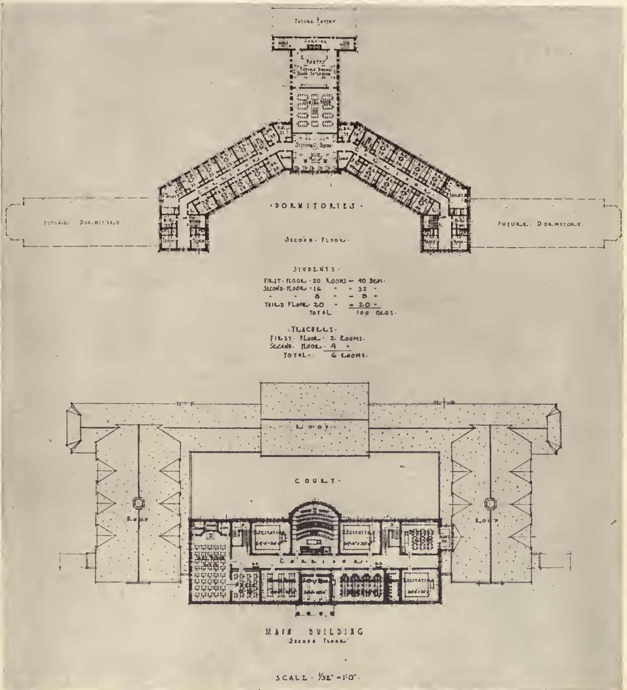
COMPETITION FOR THE STATE NORMAL SCHOOL, NEW BRITAIN, CONN. PRIZE WINNING DESIGN—GUILBERT & BETELLE, ARCHITECTS
