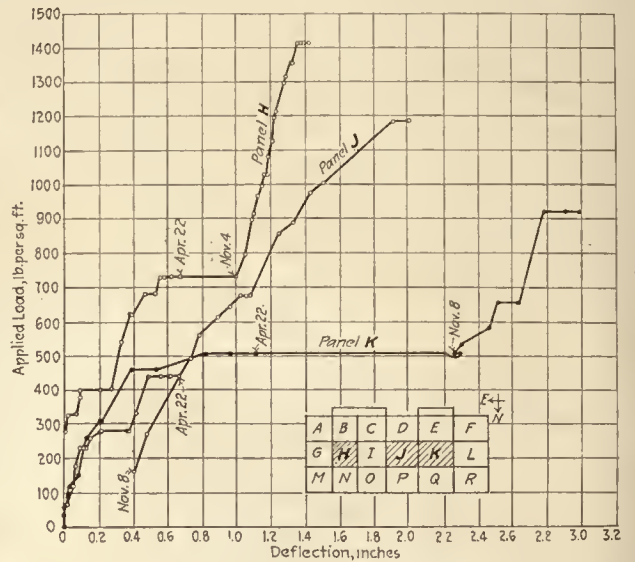
FIG. 4. CHART SHOWING AMOUNT EACH PANEL DEFLECTED AT DIFFERENT LOADINGS
