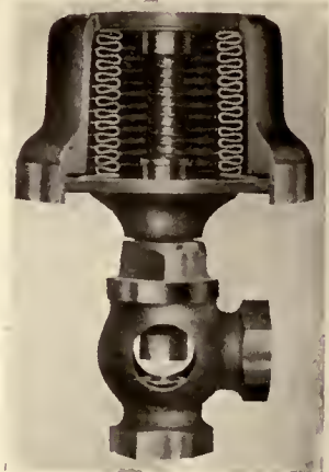
FIG. 6. PNEUMATIC VALVE OF LATEST PATTERN, SHOWING METAL BELLOWS REPLACING RUBBER DIAPHRAGM
