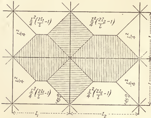
FIG. 3. DIAGRAM SHOWING AMOUNT OF LOAD ASSUMED TO BE CARRIED BY GIRDERS
