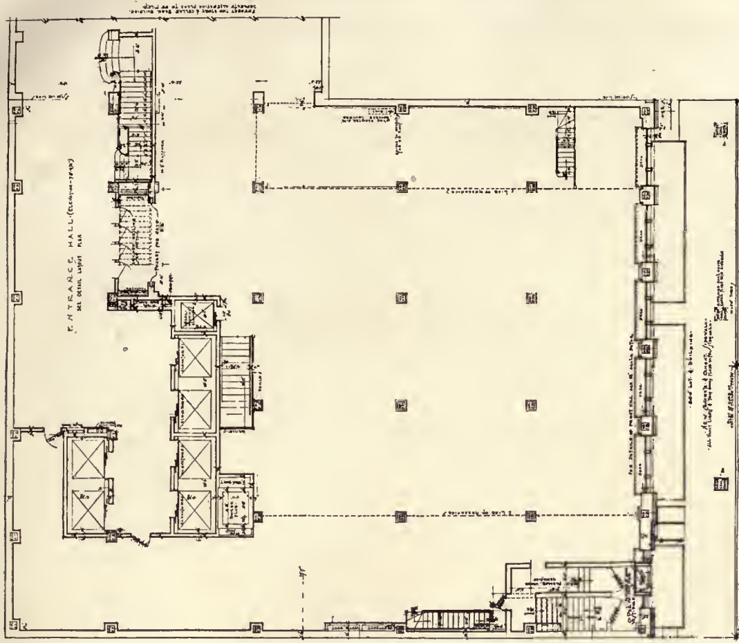
PLAN OF FIRST STORY SCALE 1/8" = 1'-0"
