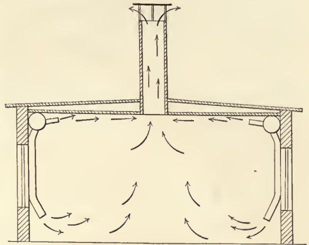
FIG. 7. TYPICAL DUCT ARRANGEMENT FOR DYE HOUSES
