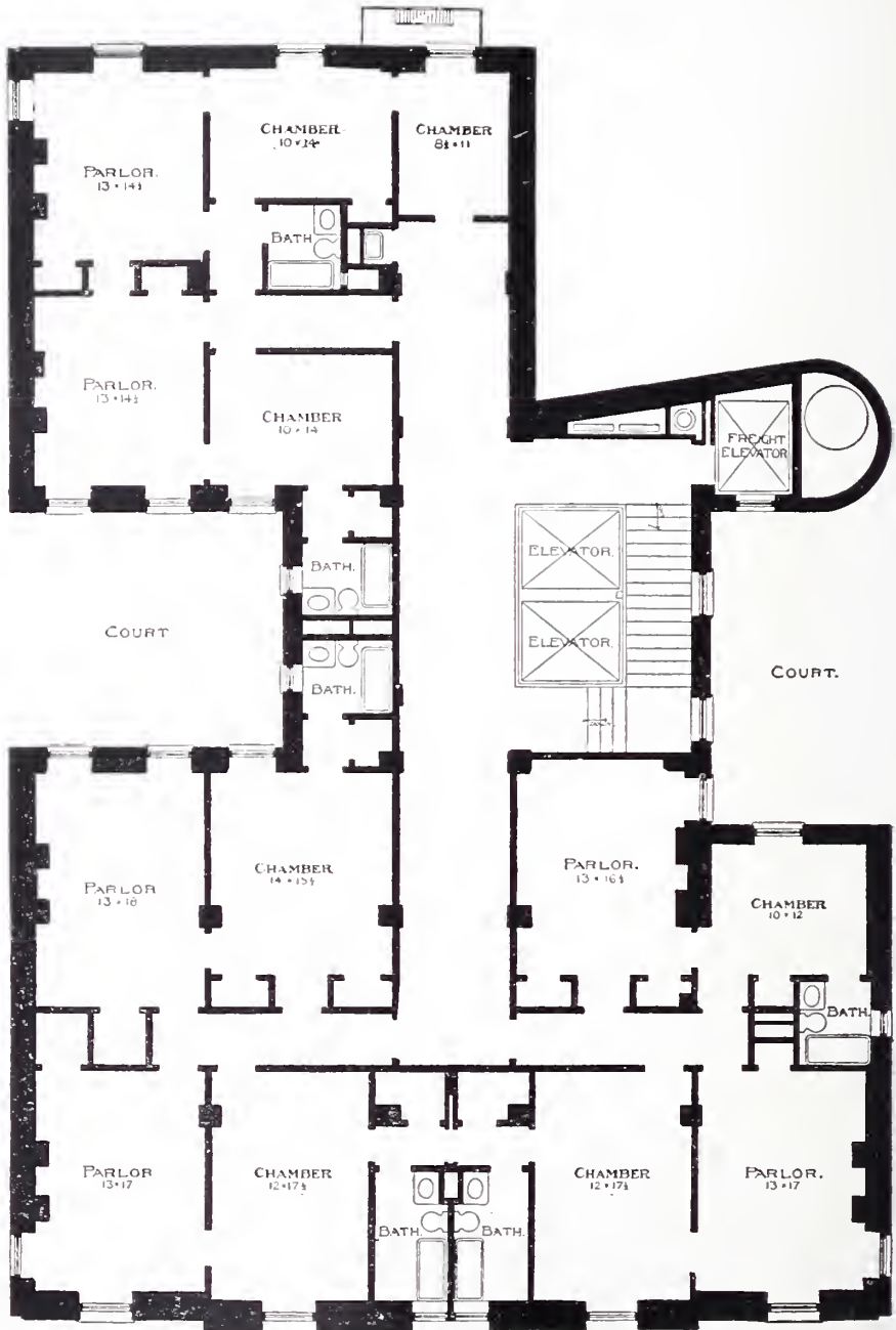
FLOOR PLAN OF THE MARTINIQUE.
