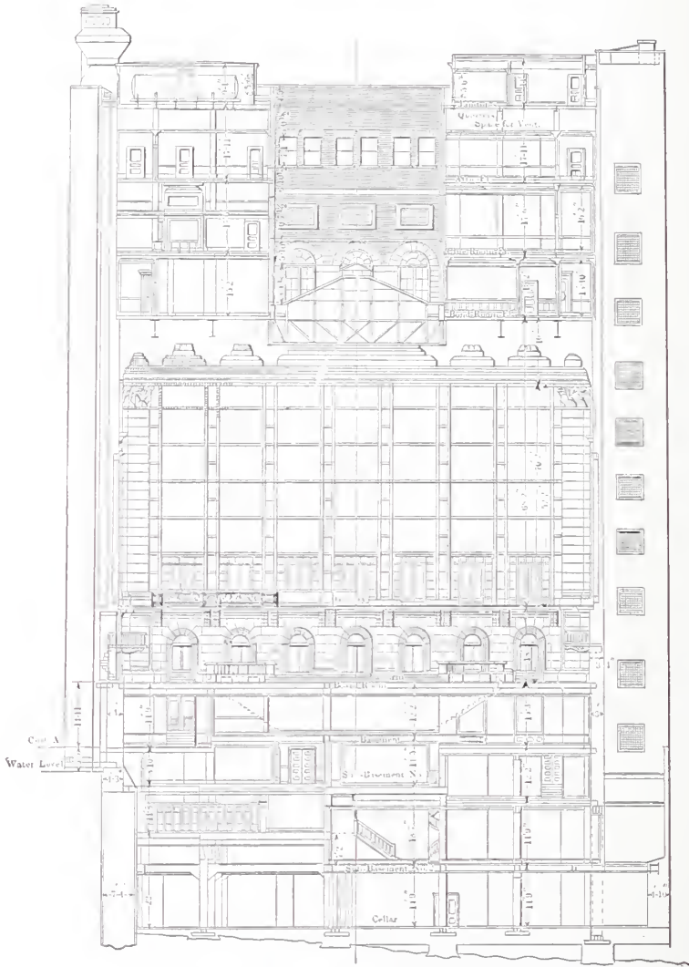
TRANSVERSE SECTION SHOWING GLASS SCREEN IN BOARD ROOM.
