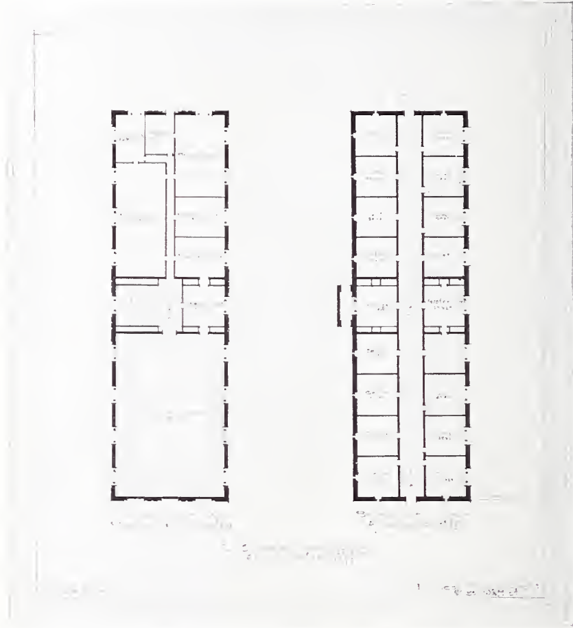
FIG. 95. PLAN OF PHYSICS AND CHEMISTRY AND ACADEMIC BUILDINGS, ANNAPOLIS.
