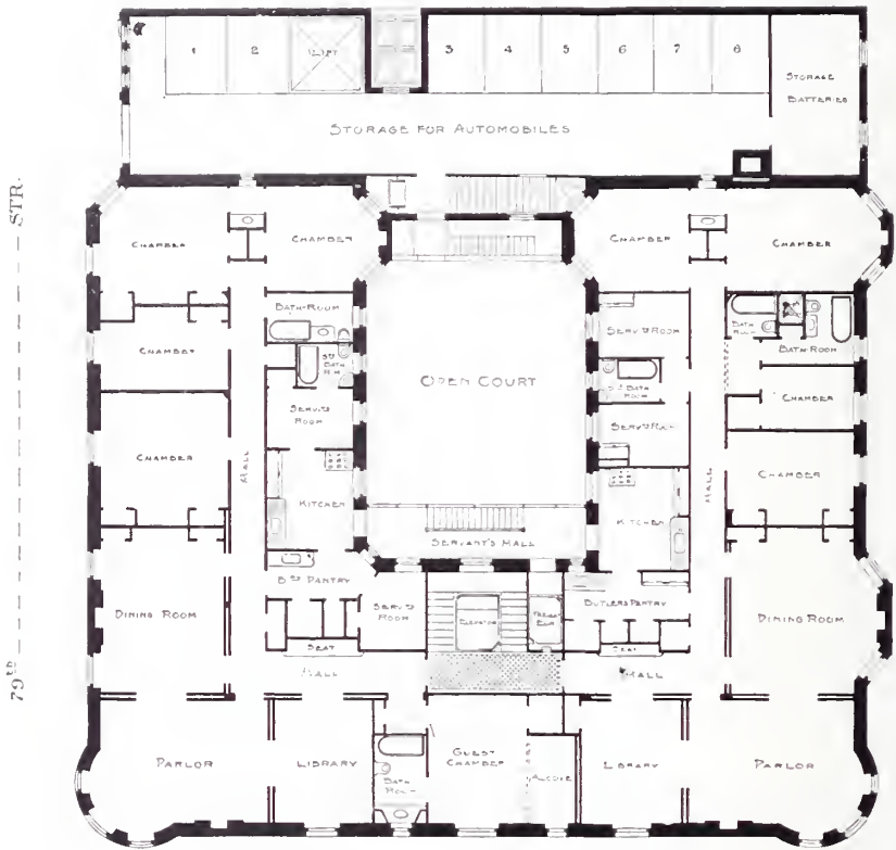
FLOOR PLAN OF AN APARTMENT HOUSE.
