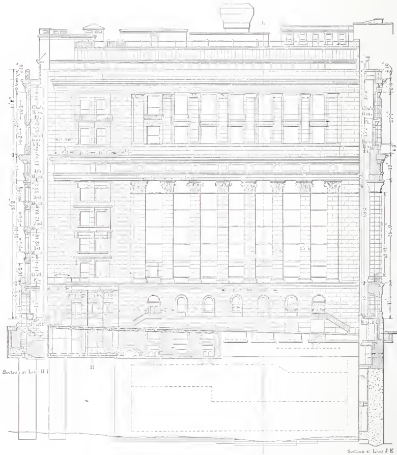
NEW STREET ELEVATION.
