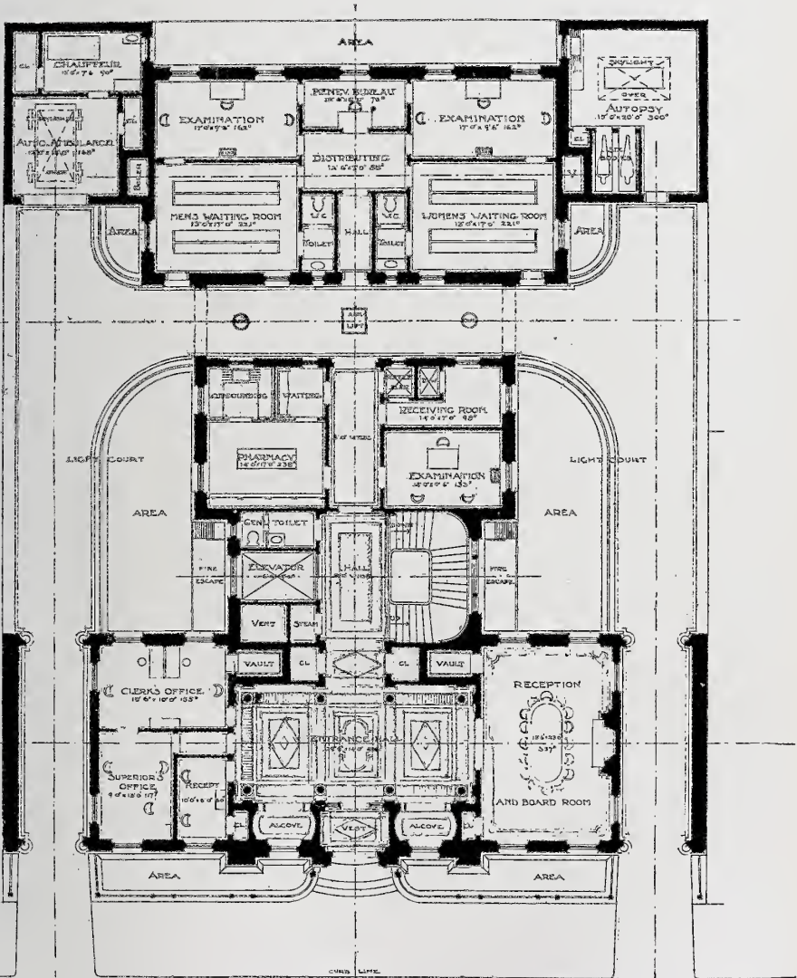
FLOOR PLAN, FRENCH HOSPITAL.
