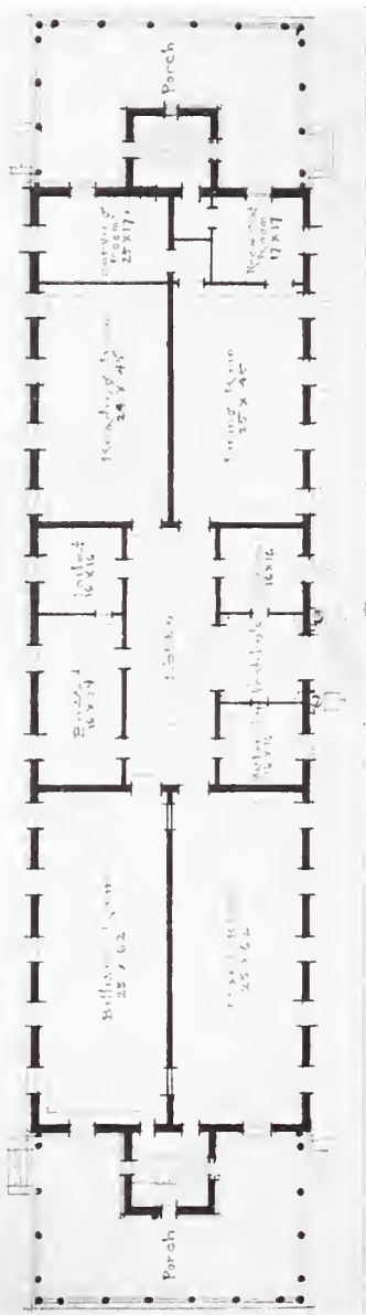
FIG. 90. PLAN OF FIRST FLOOR, OFFICERS' MESS AND CLUB, U. S. NAVAL ACADEMY, ANNAPOLIS, MD.
