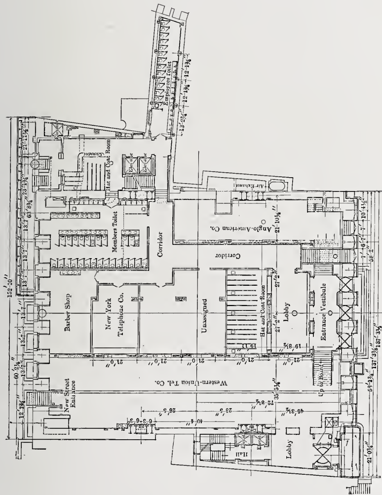
BASEMENT FLOOR.
