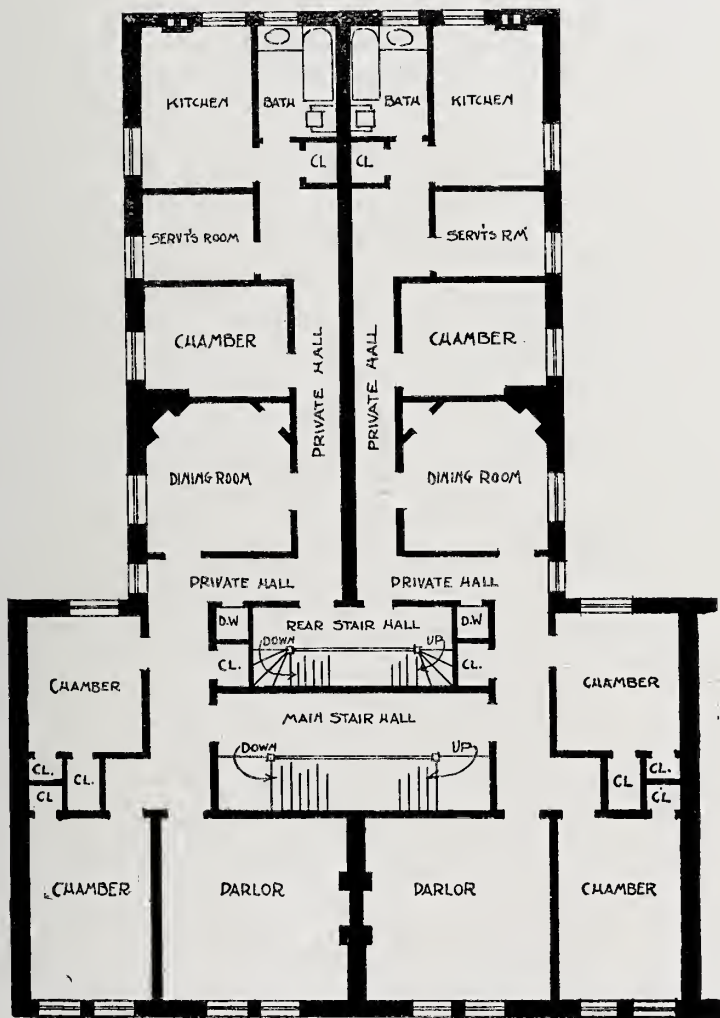
-TYPICAL-FLOOR-PLAN- STUYVESENT APARTMENT BUILDING 142 EAST 18 th ST. R.M. HUNT-ARCHITECT
