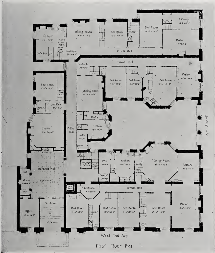
FLOOR PLAN OF APARTMENT HOUSE.
