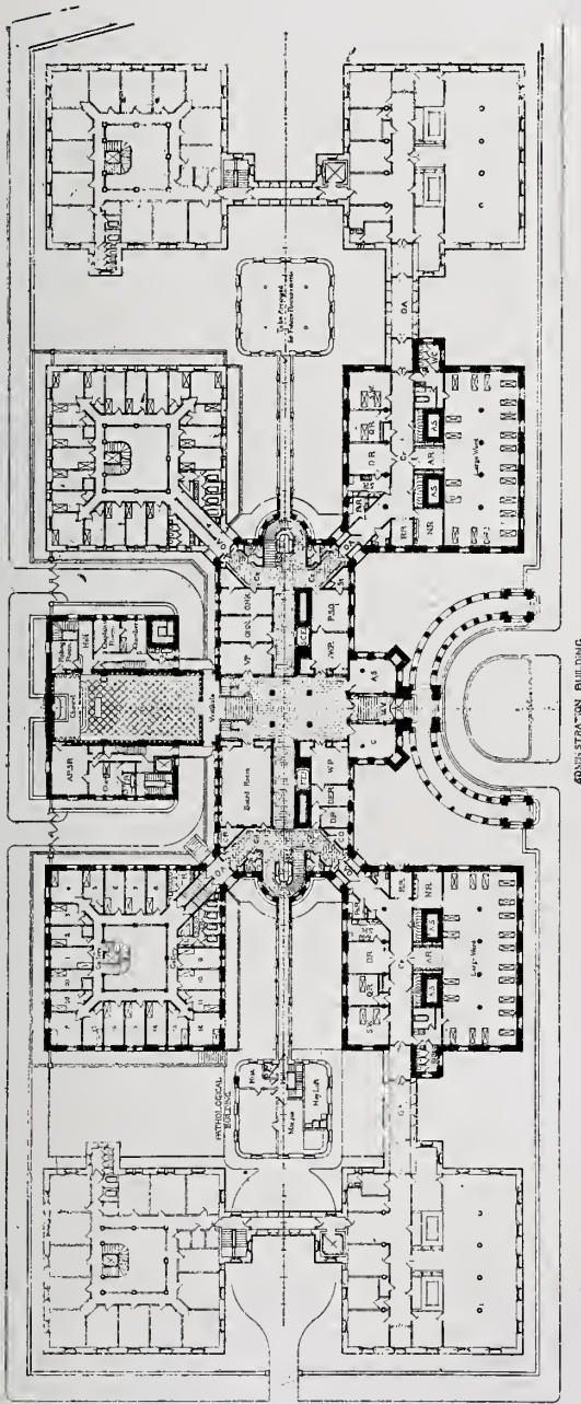
FIG. 10. GROUND FLOOR PLAN OF ST. LUKE'S HOSPITAL, CATHEDRAL HEIGHTS, NEW YORK CITY.
