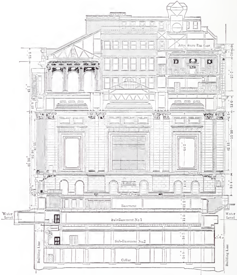
LONGITUDINAL SECTION SHOWING BULLETIN BOARD IN CENTER PANEL OF BOARD ROOM WALL.
