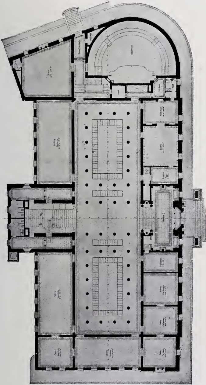
FIG. 6. PLAN OF THE GROUND FLOOR OF THE CORCORAN GALLERY OF ART, WASHINGTON, D. C.
