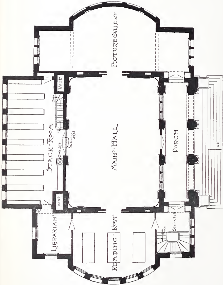
FIG. 23. PLAN OF THE LAWRENCE LIBRARY, PEPPERELL, MASS. Ernest Flagg and W. B. Chambers, Architects.
