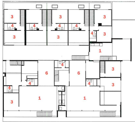
LEVEL TWO
