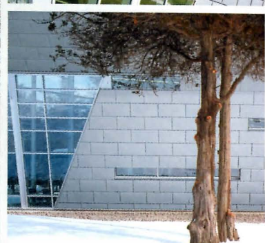
Loyalist College, Belleville, Ontario, Canada; Architect: Stephen Teeple Architects, Toronto, Ontario, Canada; Flat Lock Interlocking Wall Tiles; Fabrication and Installation: Semple Gooder, Toronto, Ontario, Canada
