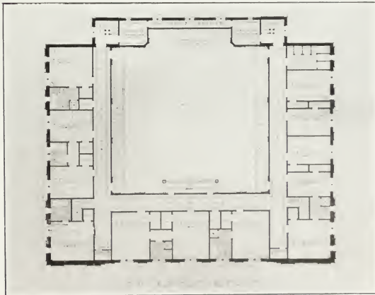
Third Floor Plan, Elks' Building Berkeley, Cal. Wm. Walter H. Russell, Jr., Architect, Berkeley, Cal.
