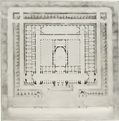
Building for the Supreme Court of the United States Ernest E. Wehr, Placed Fourth, Scholastic Competition First Medalist, S. B. A. A. Arch. Bruce Bangoris
