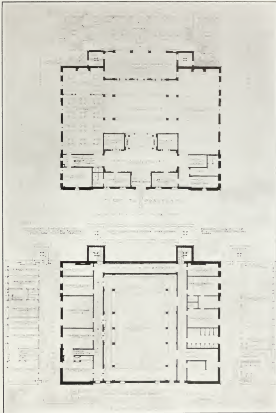
First and Basement Floor Plans, Elks' Building, Berkeley, Cal. By Walter H. Rasmussen, Jr., Architect, Berkeley, Cal.
