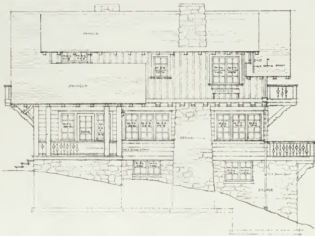
NORTH ELEVATION SCALE 1/4" = 1'-0"
