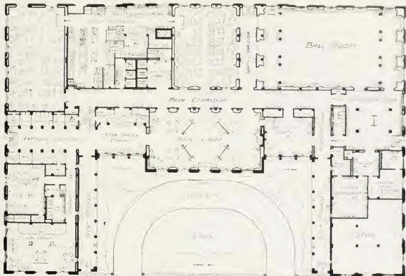
First Floor Plan 1924-25 Hotel Oakland
